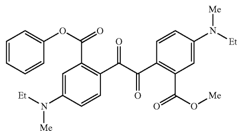
exemplary compound (98)
