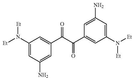
exemplary compound (95)
