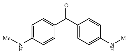
exemplary compound (5)
