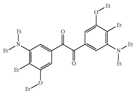
exemplary compound (96)
