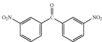
Comparative Example 9
