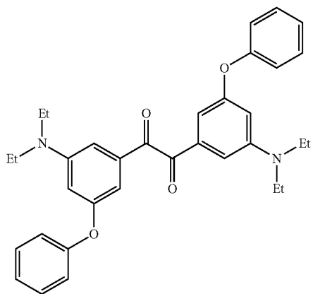
exemplary compound (95)
