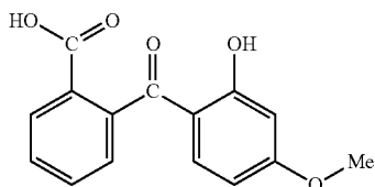
Comparative Example 8
