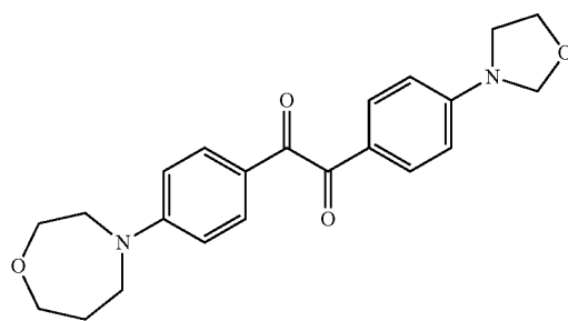
exemplary compound (100)
