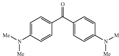
exemplary compound (7)
