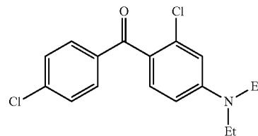
exemplary compound (9)
