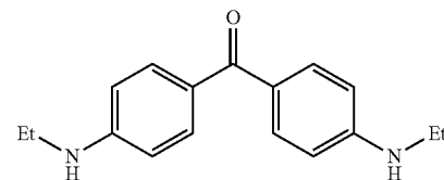
exemplary compound (8)
