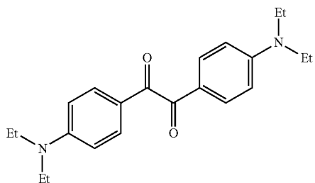
exemplary compound (92)
