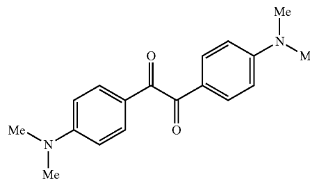
exemplary compound (4)
