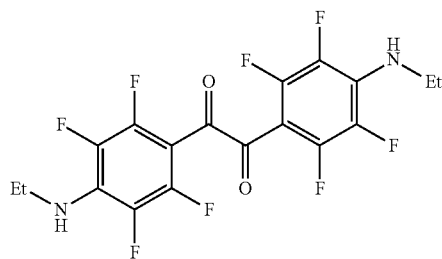
exemplary compound (99)
