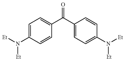
exemplary compound (2)
