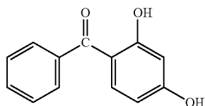
Comparative Example 7
