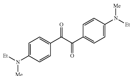
exemplary compound (97)
