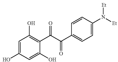
exemplary compound (92)
