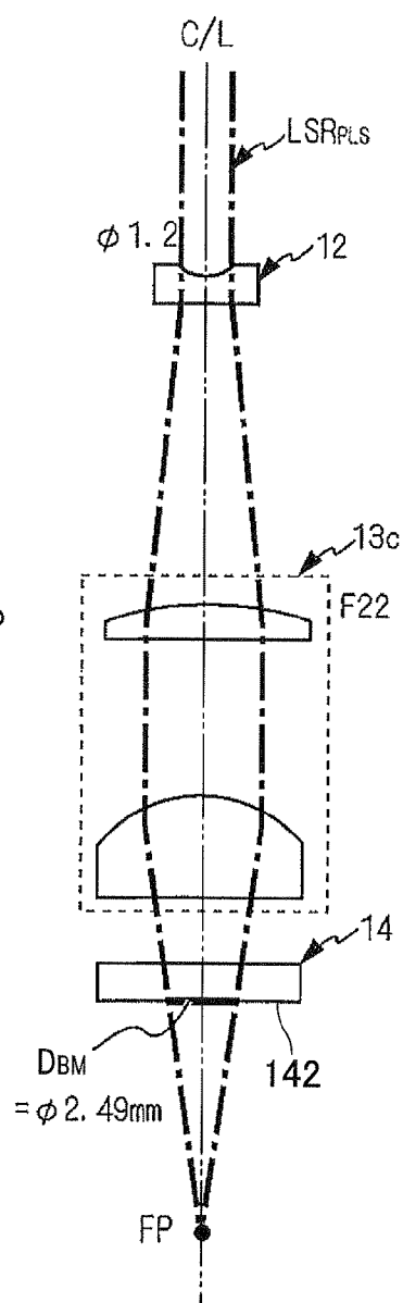
FOCUSING OPTICAL SYSTEM c
