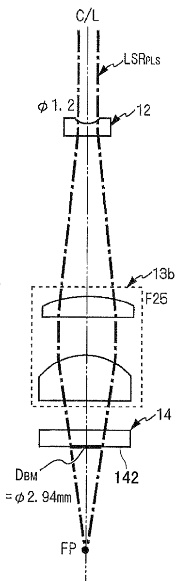
FOCUSING OPTICAL SYSTEM b
