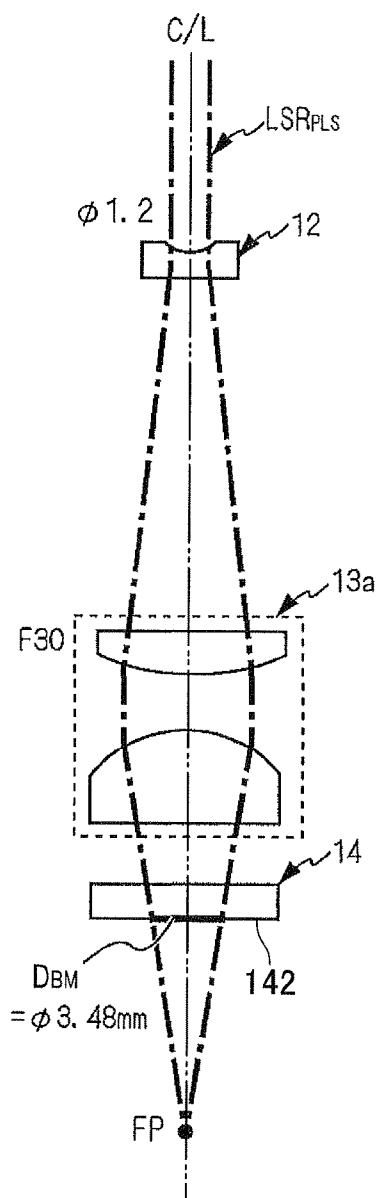
FOCUSING OPTICAL SYSTEM a
