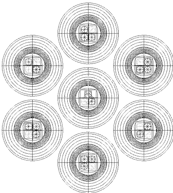
Figure 2. 7-cavity RGB LED light engine array
