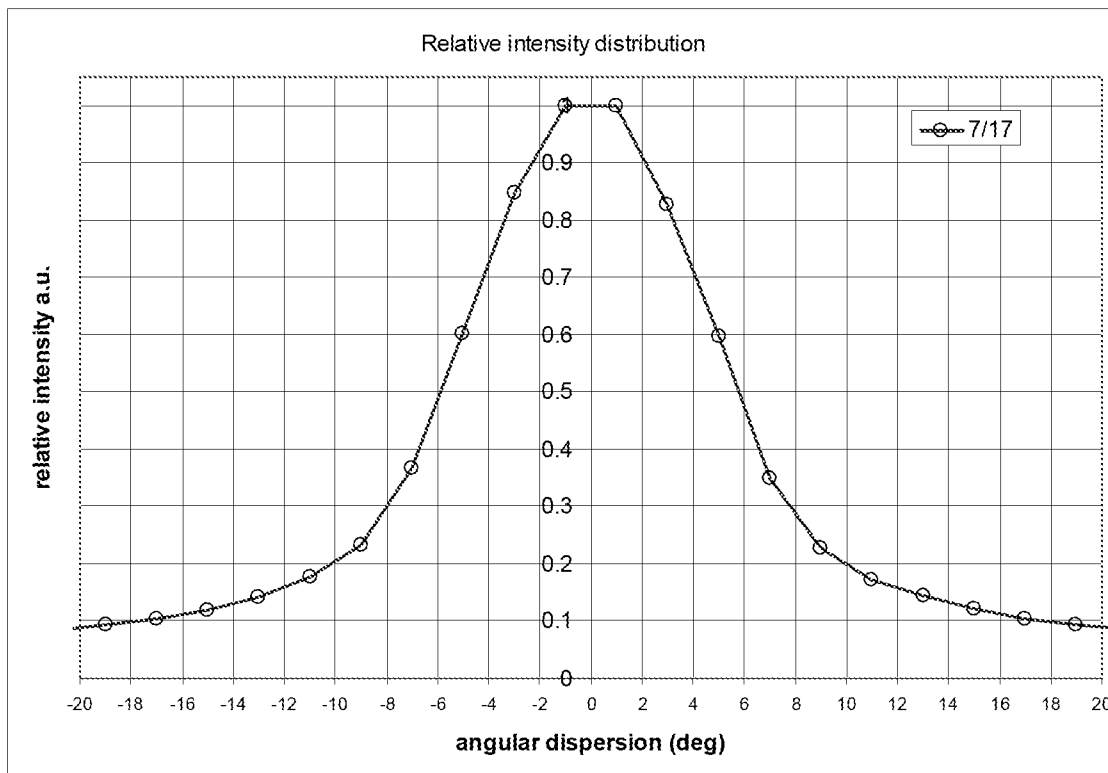
Figure 4. Intensity distribution of an 11° Beam, and 35° Field.
