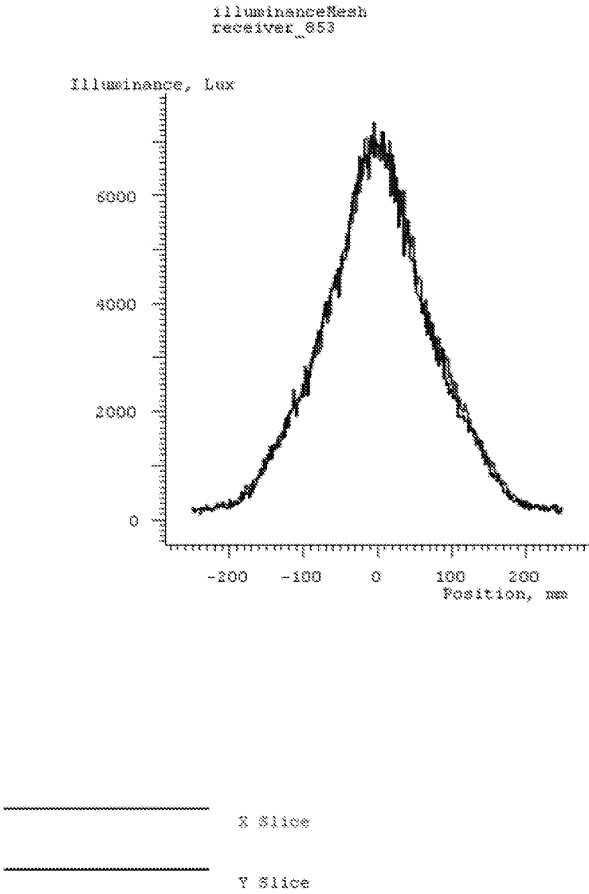
Figure 5. Illuminance distribution at 1 meter from a 7-cavity LED array source and optic
