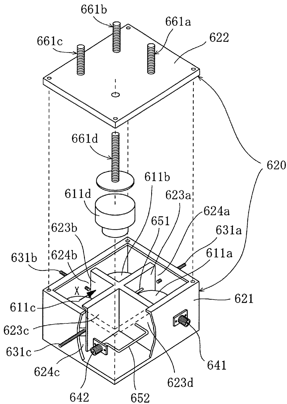
FIG. 24 PRIOR ART
