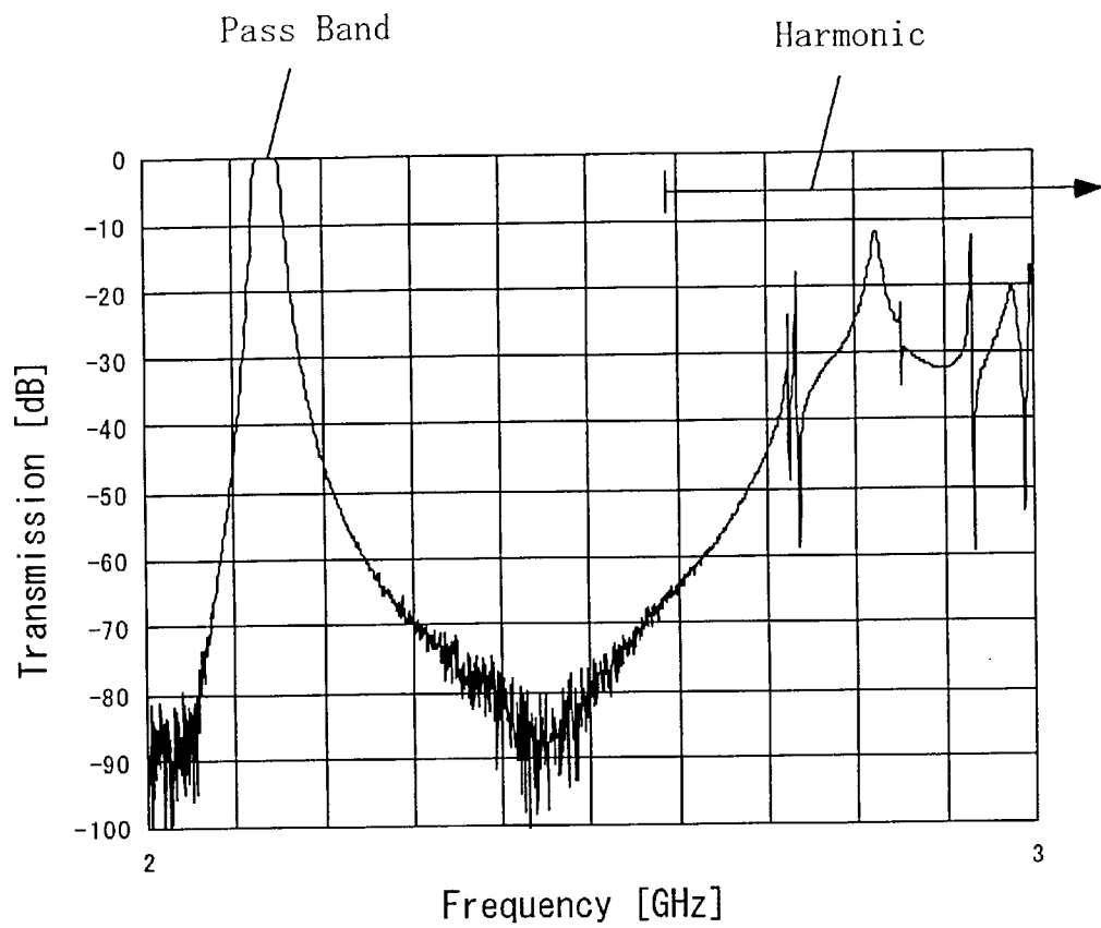
FIG. 25 PRIOR ART
