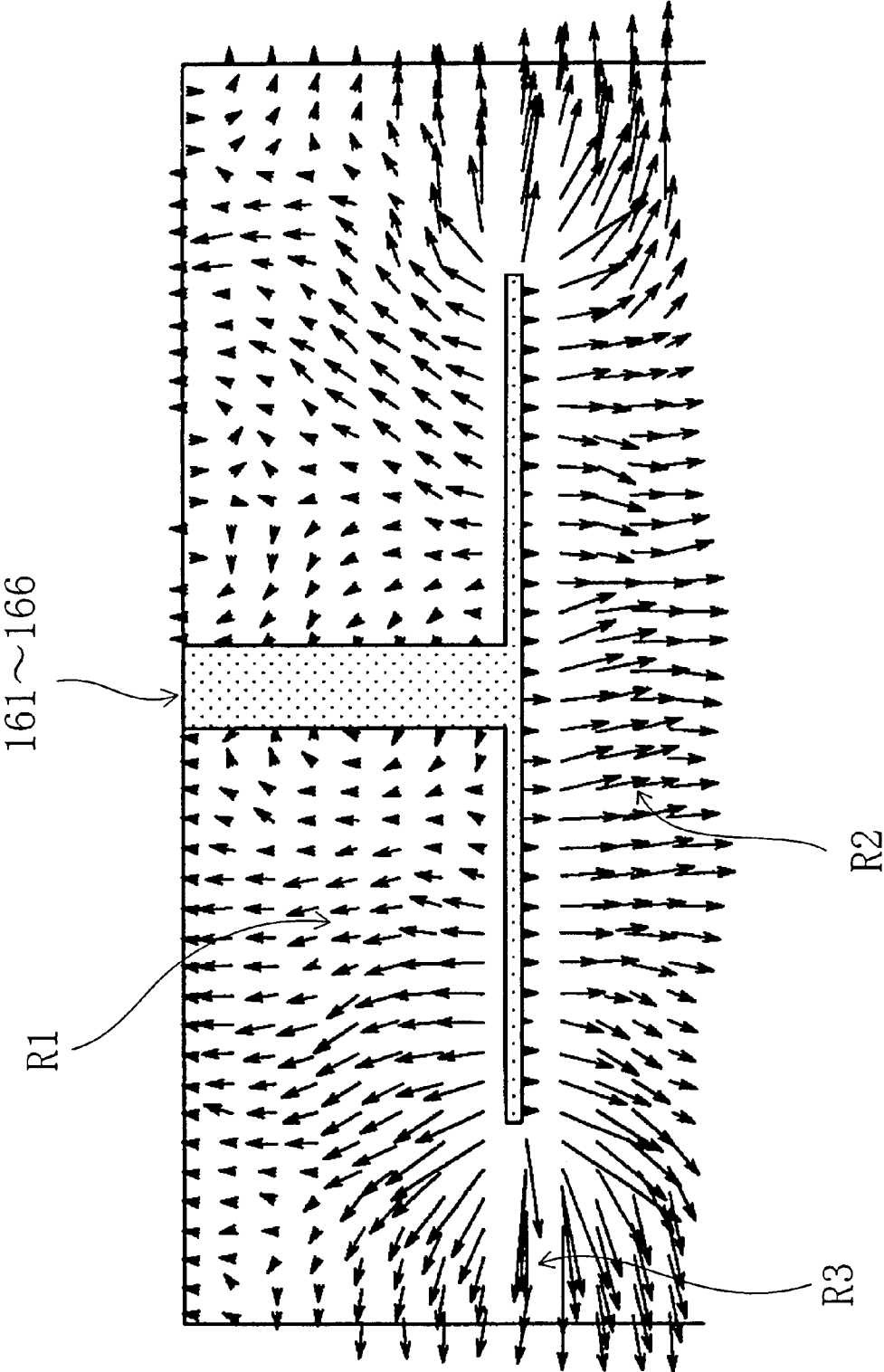
FIG. 22 PRIOR ART
