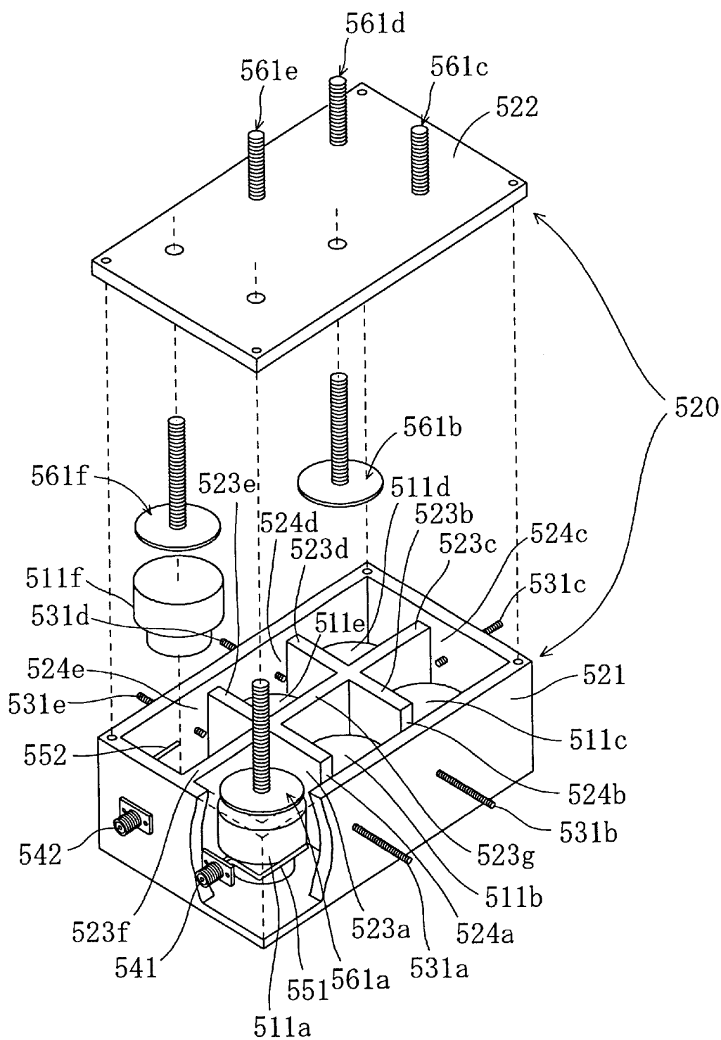
FIG. 21 PRIOR ART
