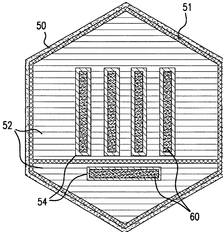
SUBMOUNT
