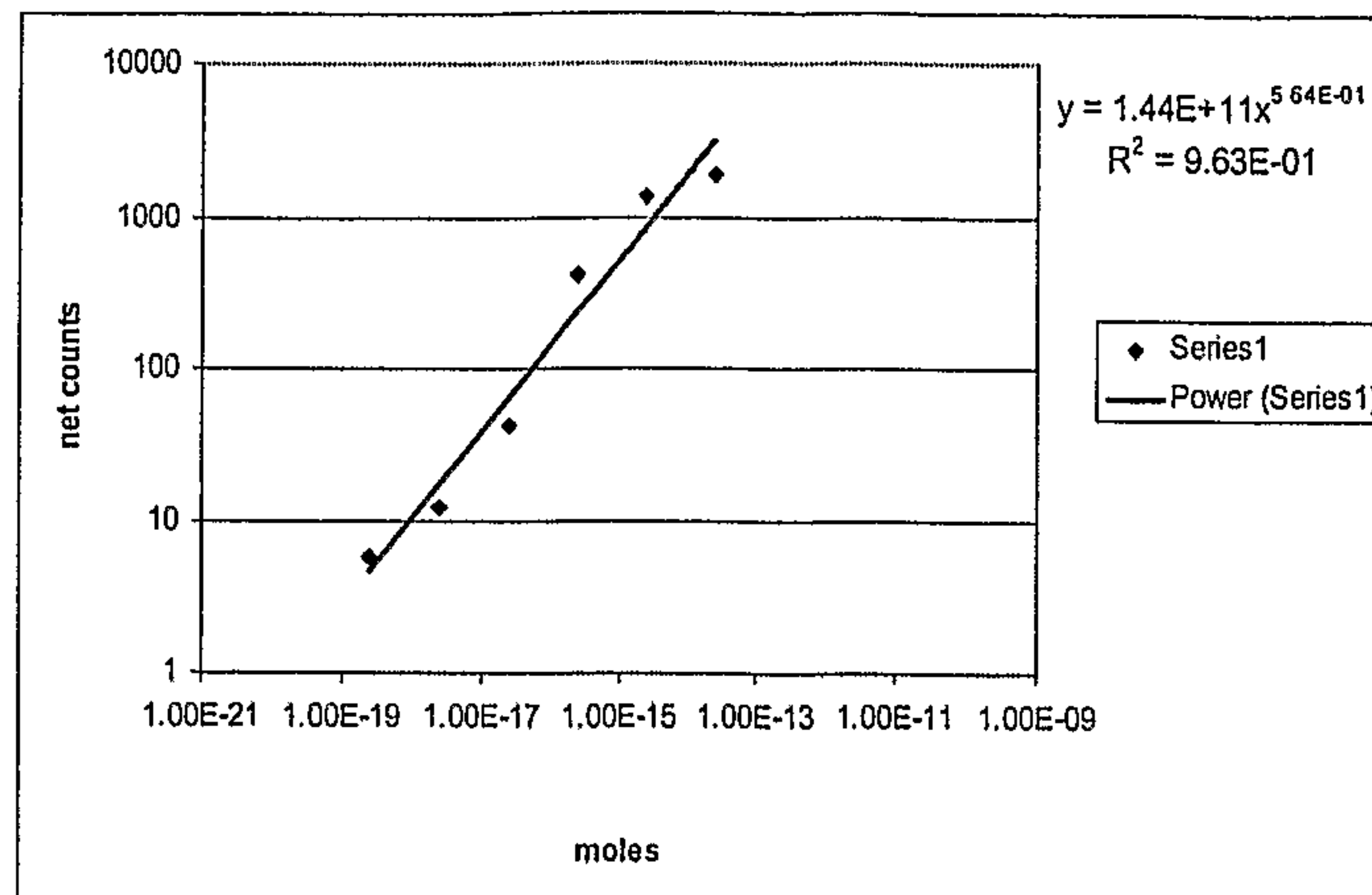
Figure 8 LOD let-7 (1496-78-01R)
