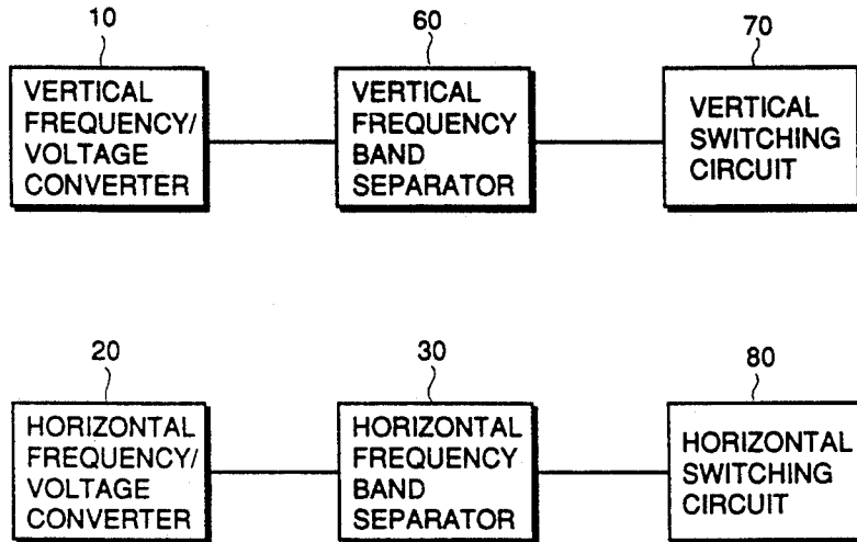
FIG.1 (PRIOR ART)
