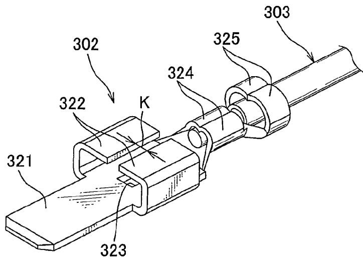
FIG. 6 (PRIOR ART)
