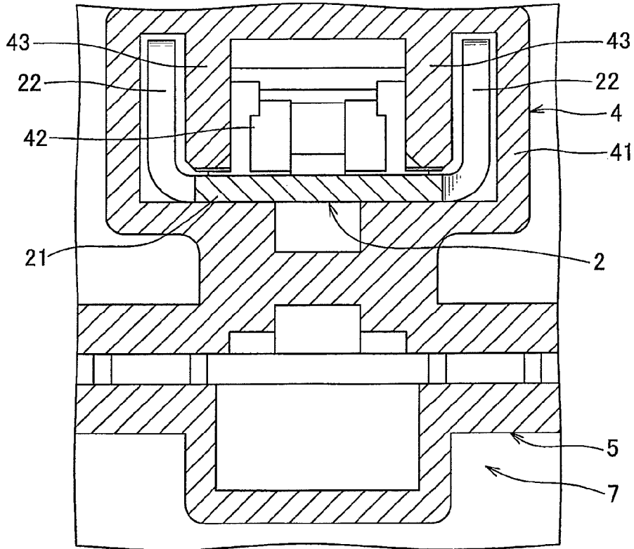
FIG. 6 (PRIOR ART)
