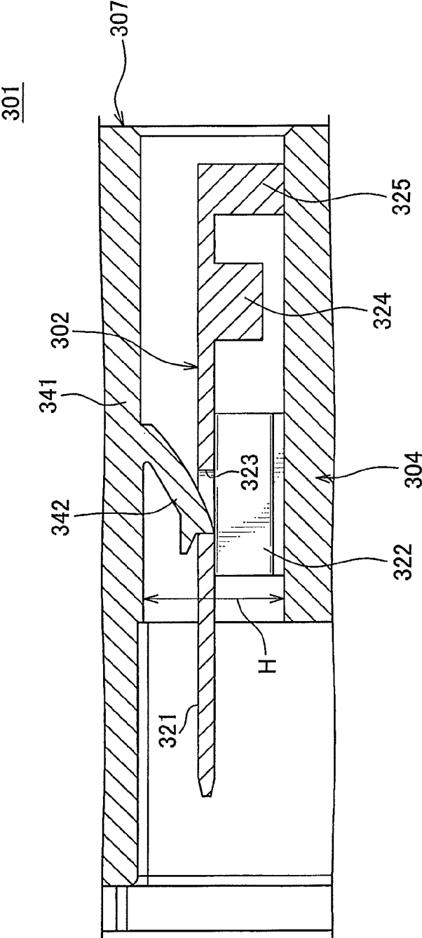
FIG. 7 (PRIOR ART)
