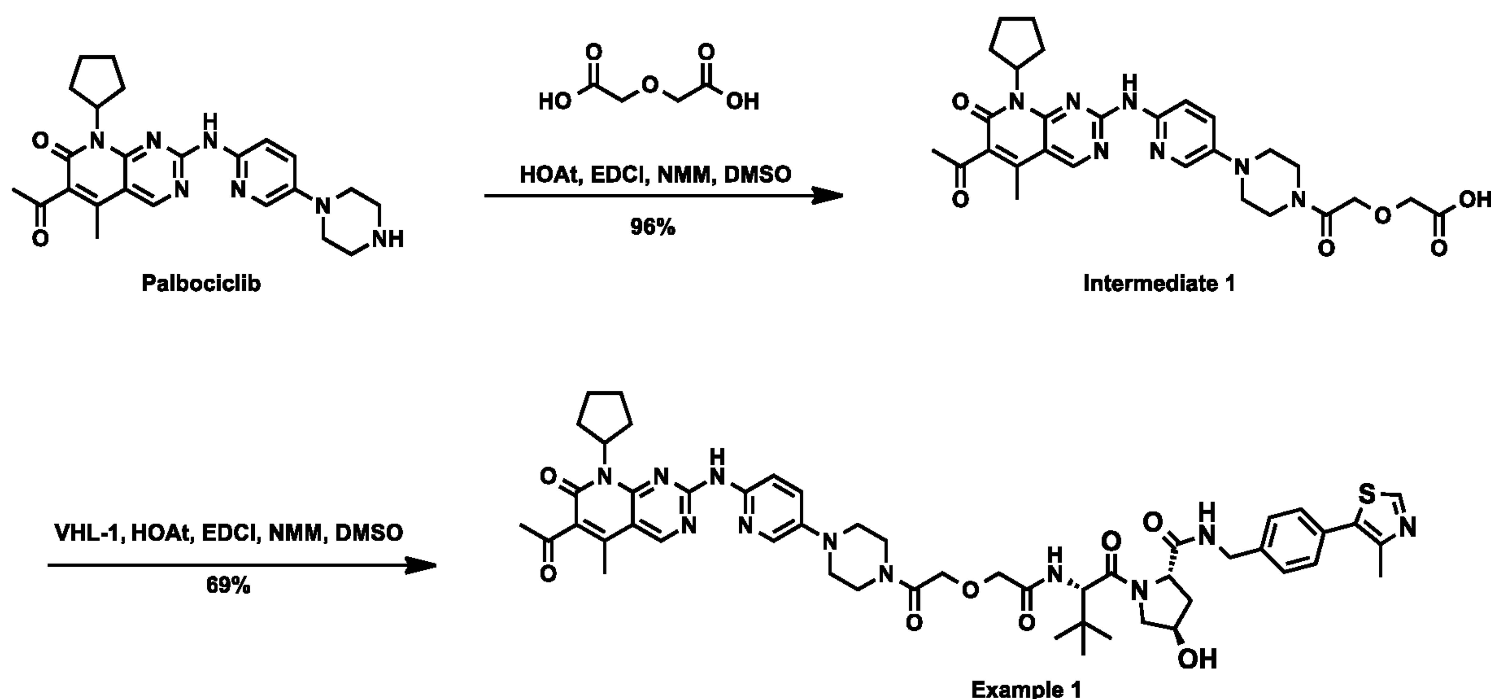
Scheme 1: Synthesis of example 1
