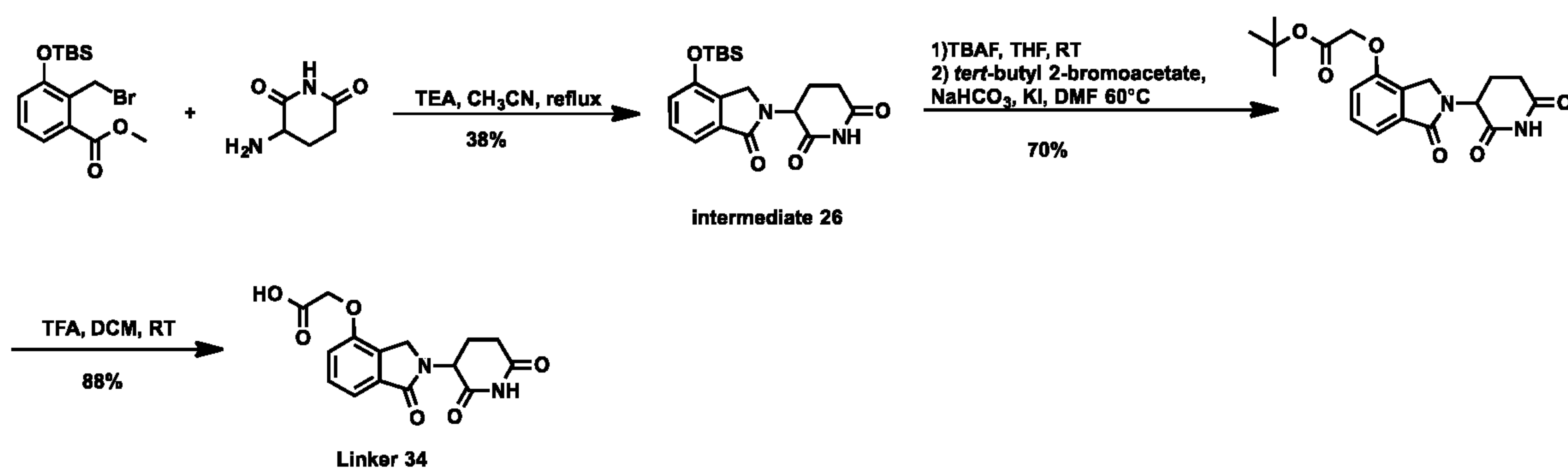
Scheme 29: Synthesis of Linker 34
