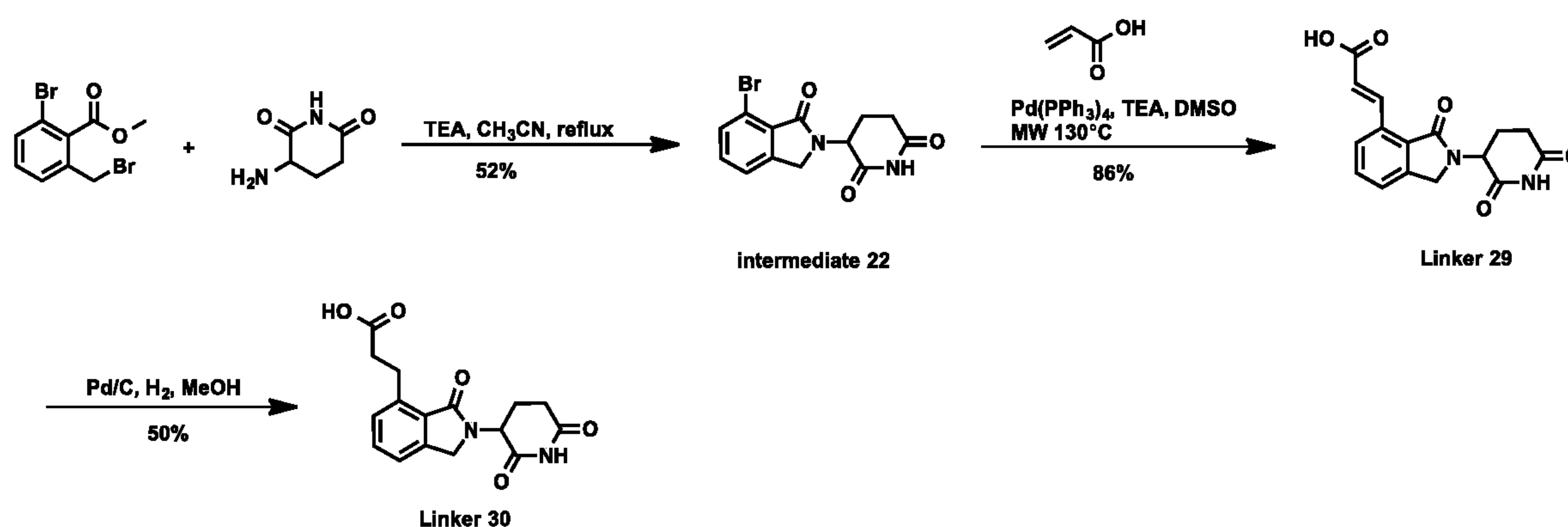
Scheme 25: Synthesis of Linker 29 and 30
