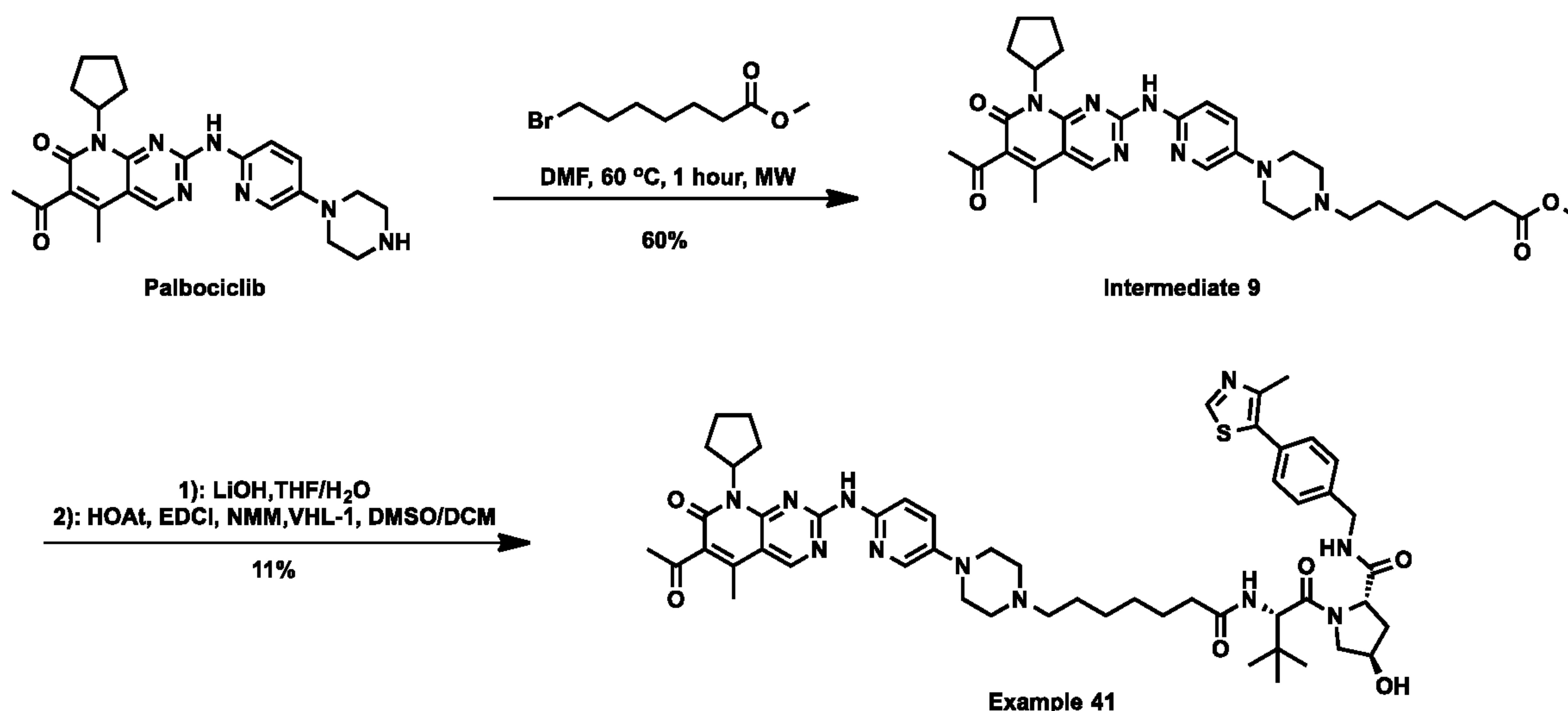
Scheme 13: Synthesis of example 41
