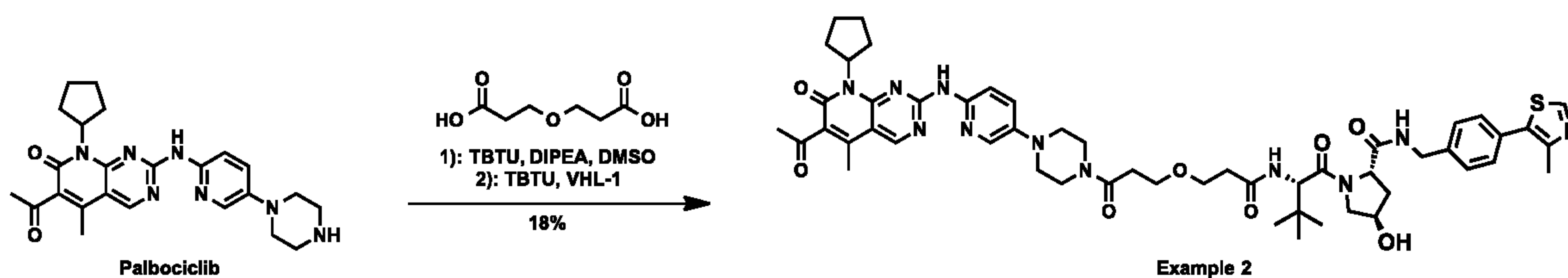
Scheme 2: Synthesis of example 2
