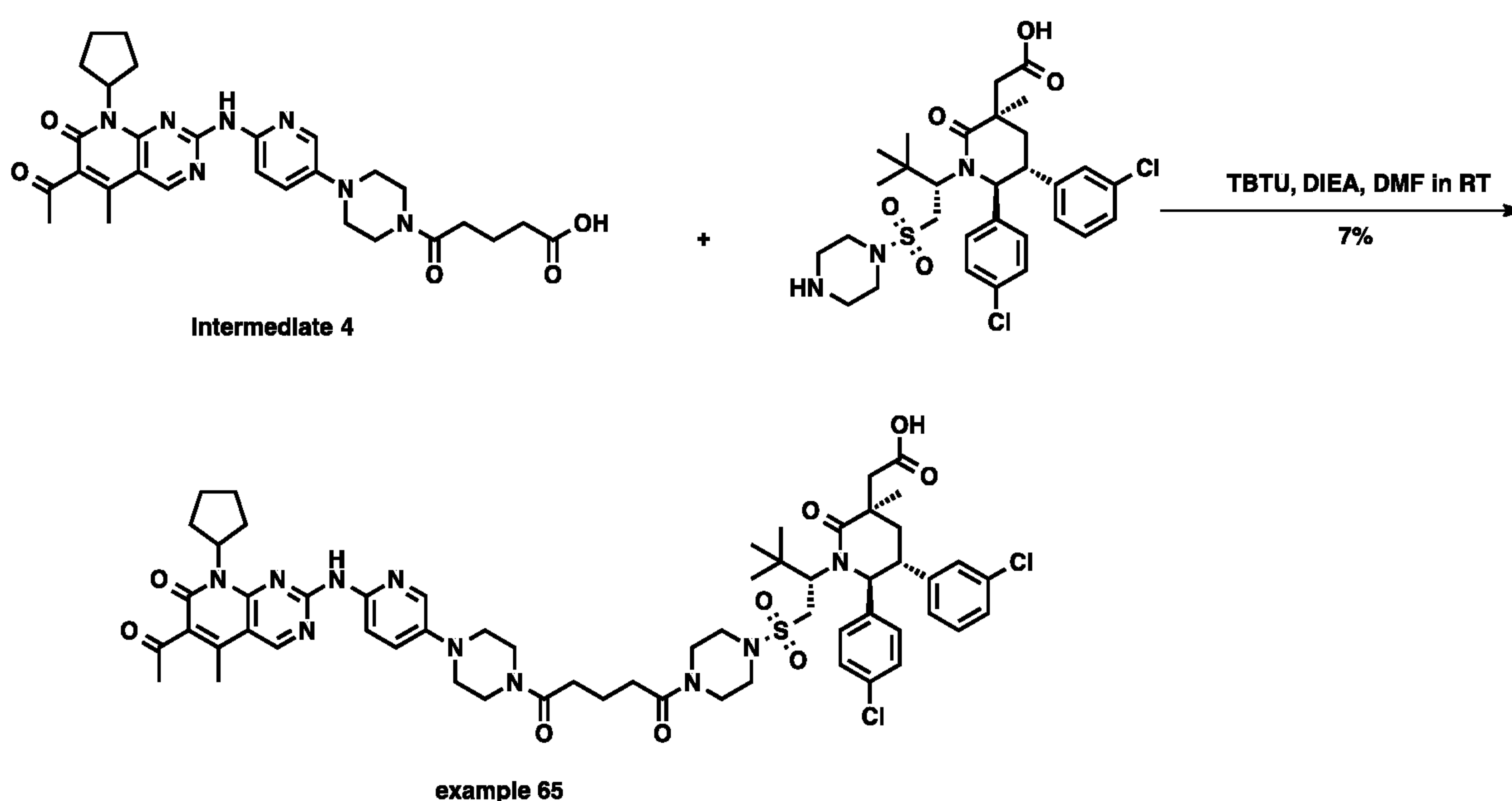
Scheme 33: synthesis of example 65
