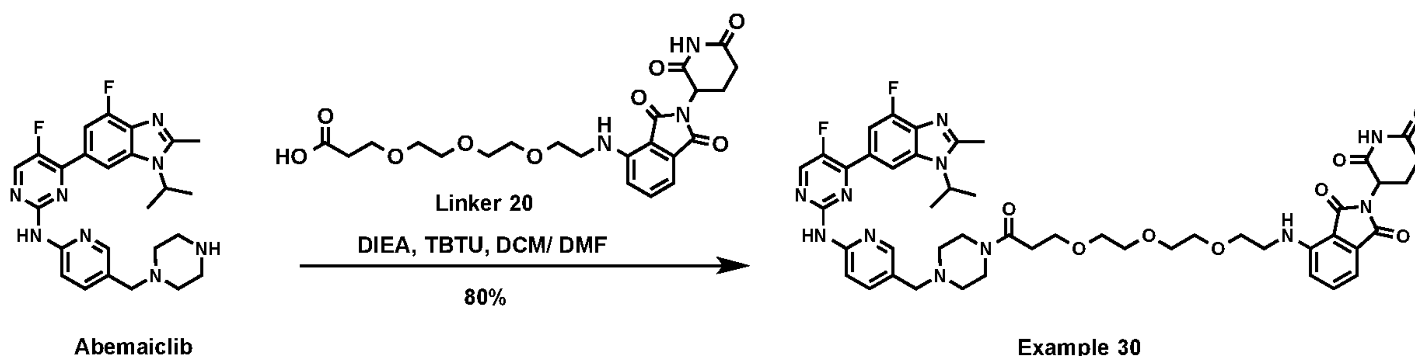
Scheme 6: Synthesis of example 30
