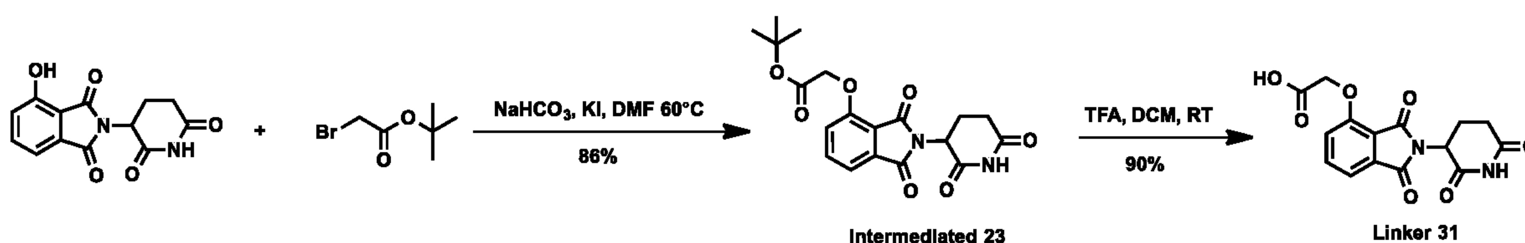
Scheme 26: Synthesis of Linker 31
