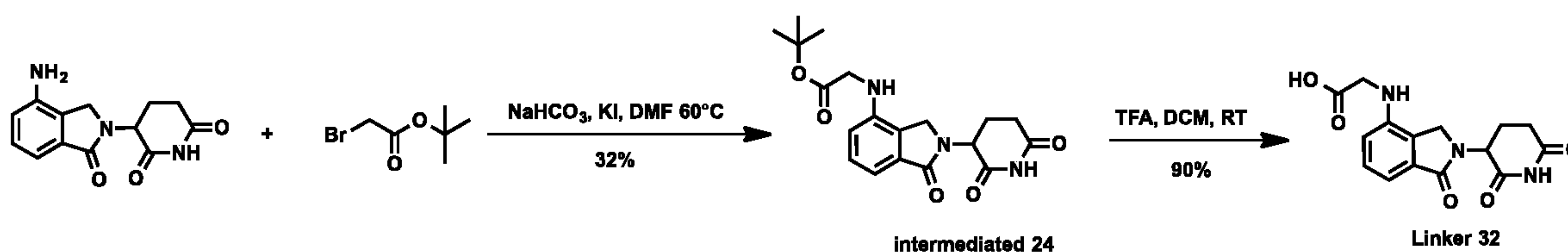
Scheme 27: Synthesis of Linker 32
