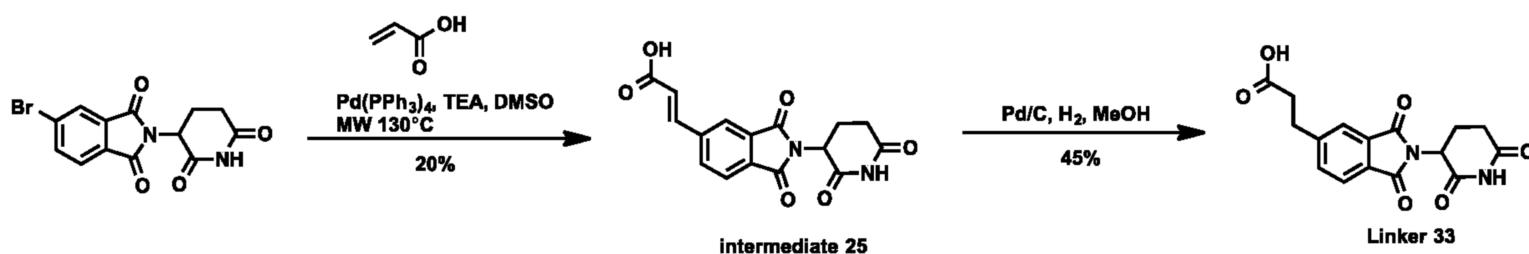
Scheme 28: Synthesis of Linker 33
