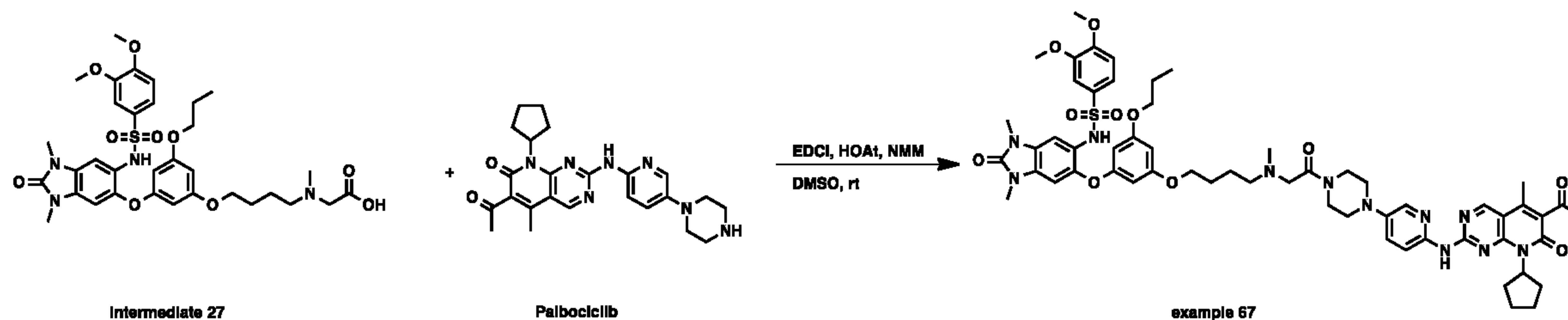
Scheme 35: synthesis of example 67
