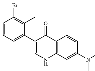
3-(3-Bromo-2-methyl-phenyl)-7-dimethylamino-1H-quinolin-4-one
