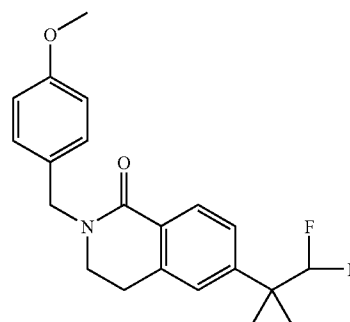
6-(1-Difluoromethyl-cyclopropyl)-2-(4-methoxy-benzyl)-3,4-dihydro-2H-isoquinolin-1-one (VII)
