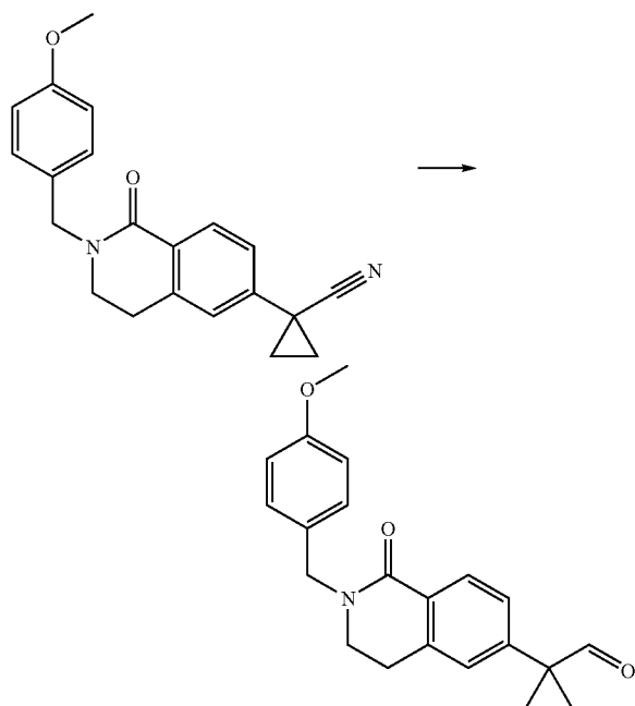
1-[2-(4-Methoxy-benzyl)-1-oxo-1,2,3,4-tetrahydro-isoquinolin-6-yl]-cyclopropanecarbaldehyde (VI)
