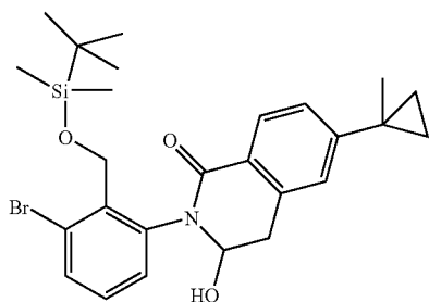
2-[3-Bromo-2-(tert-butyl-dimethyl-silanyloxymethyl)-phenyl]-3-hydroxy-7-(1-methyl-cyclopropyl)-3,4-dihydro-2H-isoquinolin-1-one
