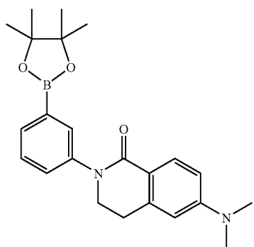
6-Dimethylamino-2-[3-(4,4,5,5-tetramethyl-[1,3,2]dioxaborolan-2-yl)-phenyl]-3,4-dihydro-2H-isoquinolin-1-one
