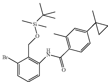
N-[3-Bromo-2-(tert-butyl-dimethyl-silanyloxymethyl)-phenyl]-2-methyl-4-(1-methyl-cyclopropyl)-benzamide
