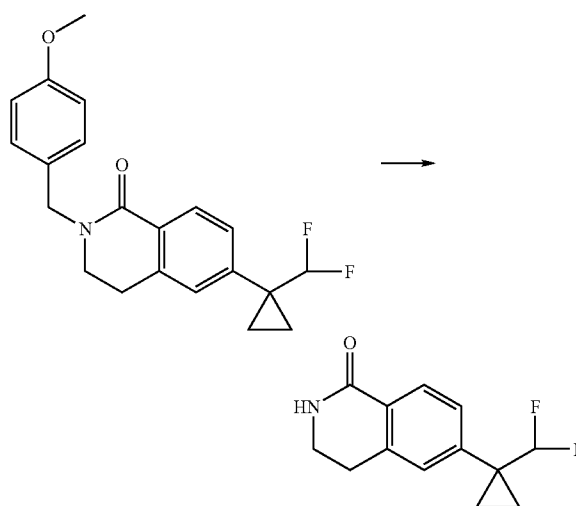
6-(1-Difluoromethyl-cyclopropyl)-3,4-dihydro-2H-isoquinolin-1-one (VIII)
