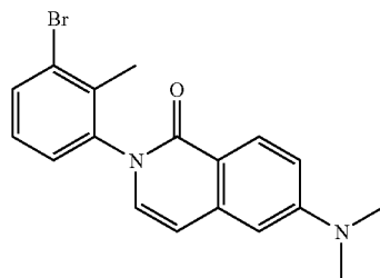
2-(3-Bromo-2-methyl-phenyl)-6-dimethylamino-2H-isoquinolin-1-one
