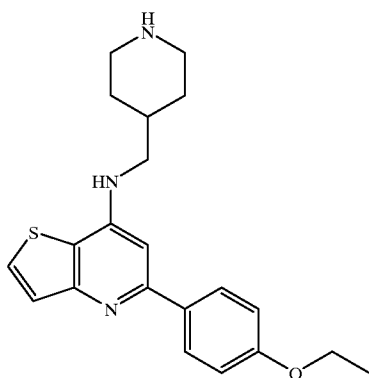
Compound 7
