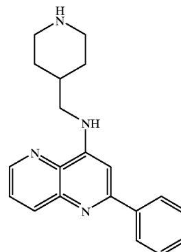
Compound 9
