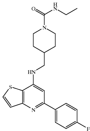
Compound 8
