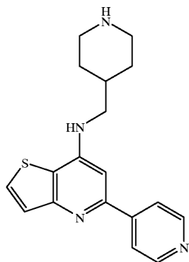
Compound 6
