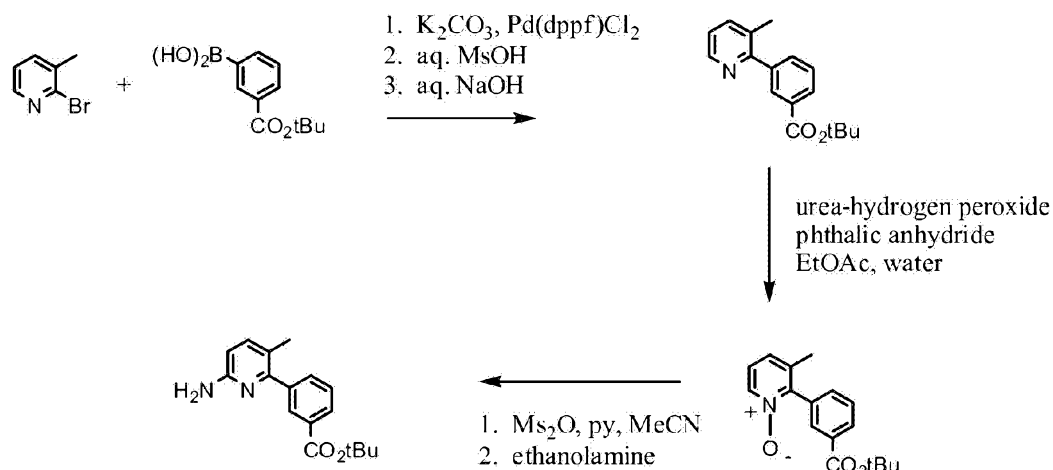
Scheme 3. Synthesis of the amine moiety.
