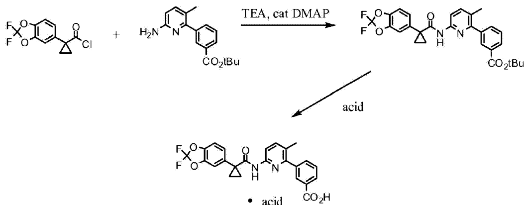
Scheme 4. Formation of an acid salt of 3-(6-(1-(2,2-difluorobenzo[d][1,3]dioxol-5-yl)cyclopropanecarboxamido)-3-methylpyridin-2-yl)benzoic acid.
