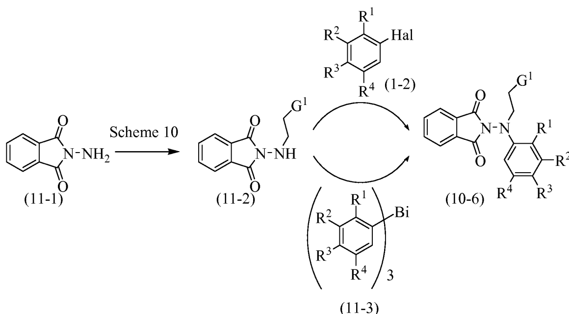
Scheme 11
