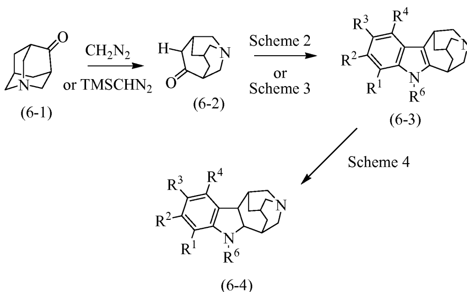
Scheme 6
