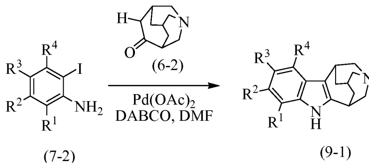
Scheme 9
