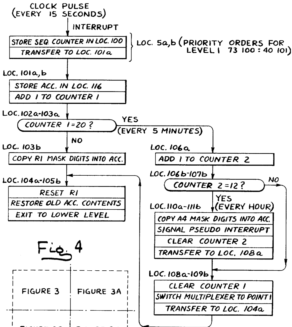
Fig. 13 LEVEL 1 CLOCK ROUTINE
