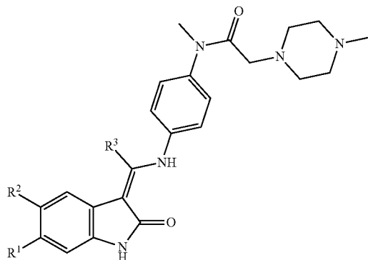
Formula I
