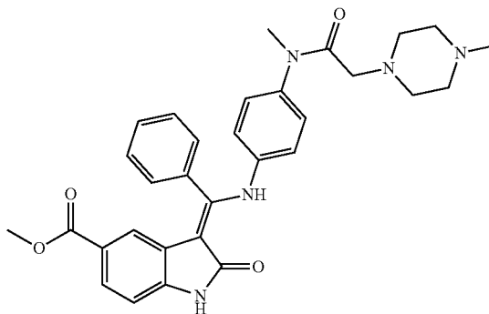
Compound 17
