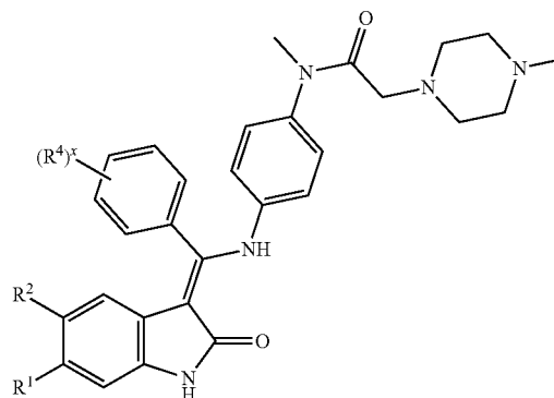
Formula III
