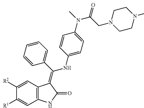
Formula II
