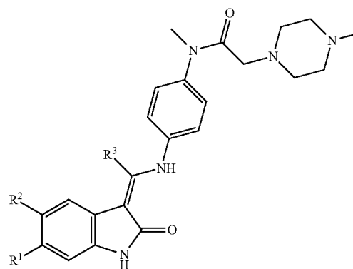
Formula I
