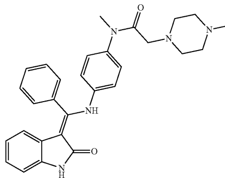
Compound 16
