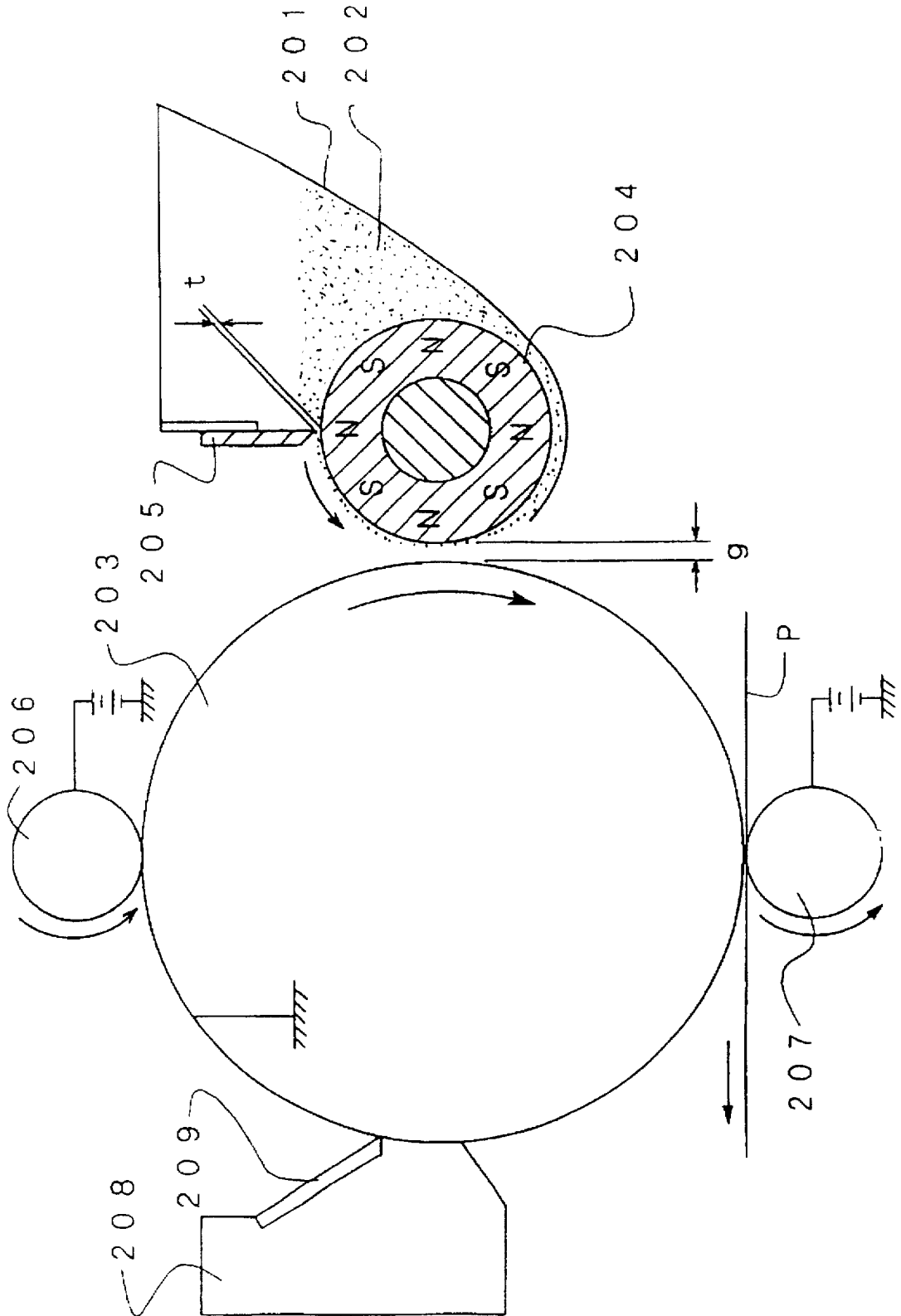
FIG. 7 (PRIOR ART)
