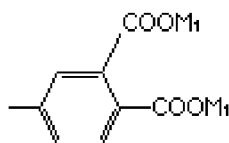
General formula (3)
