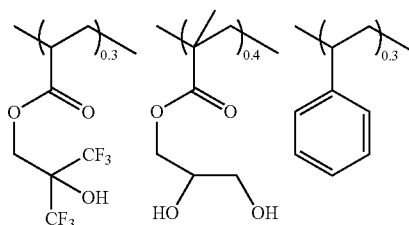
Synthesis Example 4
