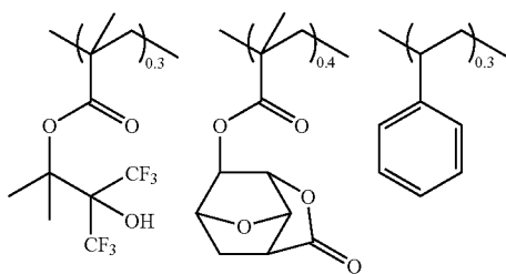
Synthesis Example 16
