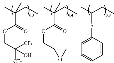
Synthesis Example 8
