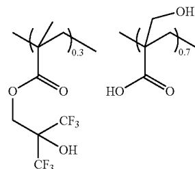
Synthesis Example 6
