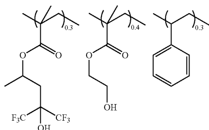
Synthesis Example 5
