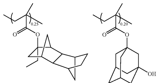
polymer 1
