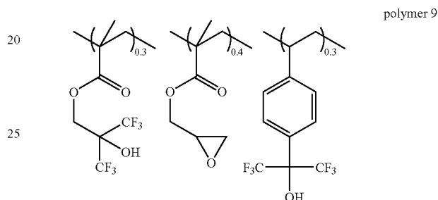
Synthesis Example 10
