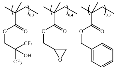
Synthesis Example 9
