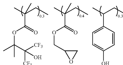
Synthesis Example 7
