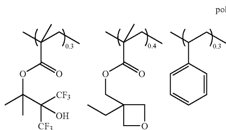
Synthesis Example 15
