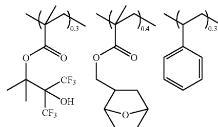
Synthesis Example 17
