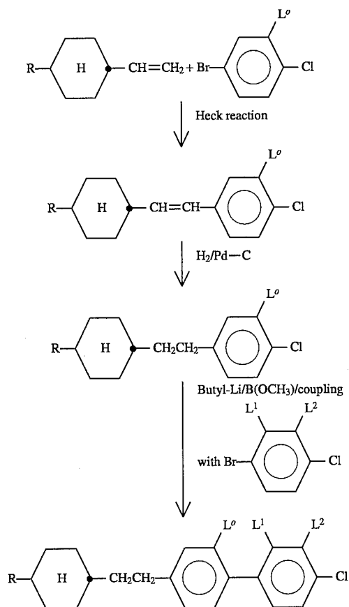
Scheme 4
