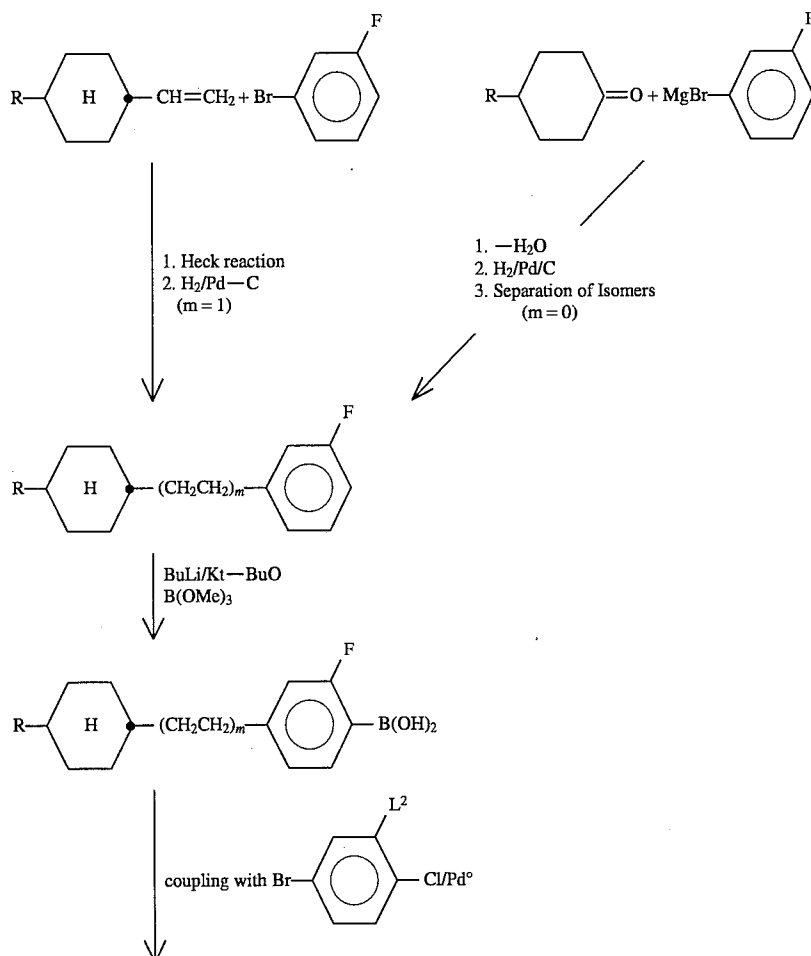
Scheme 10
