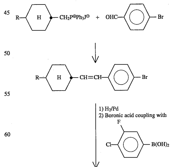
Scheme 6
