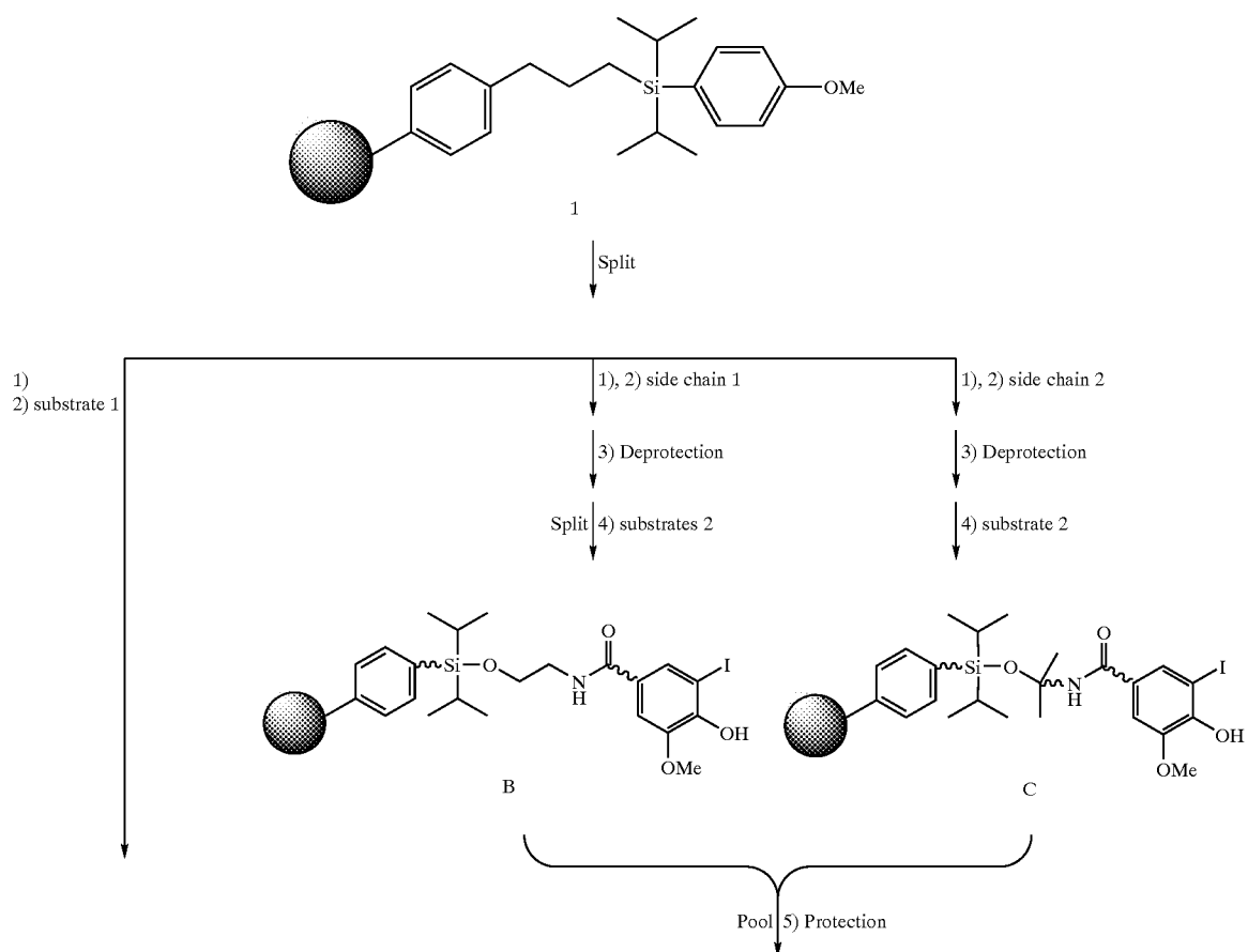
Scheme 4: Constructing C2/S2 Symmetric 2,3-distributed Benzol[b]furan Scaffold
