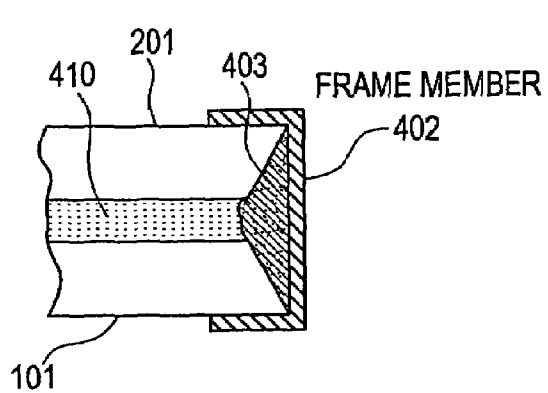
SECTIONAL VIEW OF PORTION a
