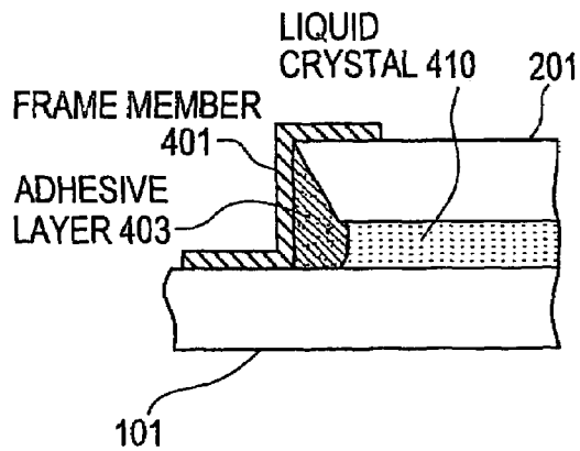
SECTIONAL VIEW OF PORTION a
