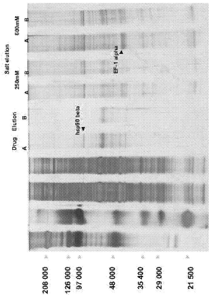
A (biotinylated incubation RC-MC-110) B (Competition 10X RC-MC110 + Biotinylated RC-MC-110)
