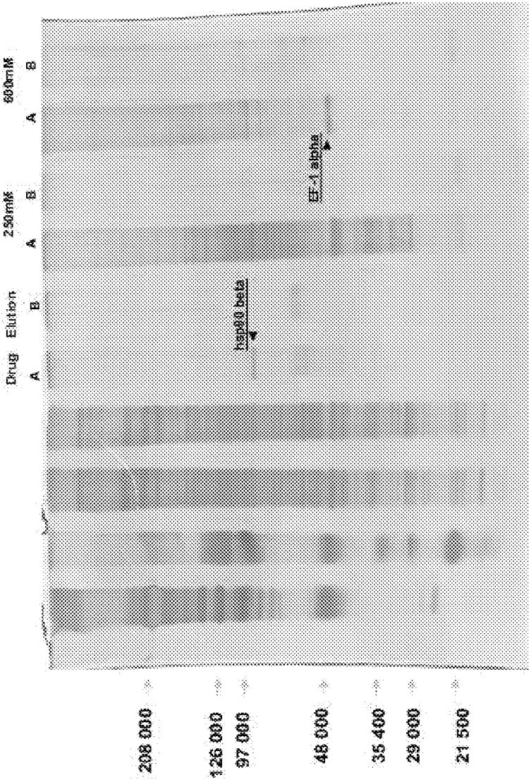
A (biotinylated incubation RC-MC-110) B (Competition 10X RC-MC110 + Biotinylated RC-MC-110)
