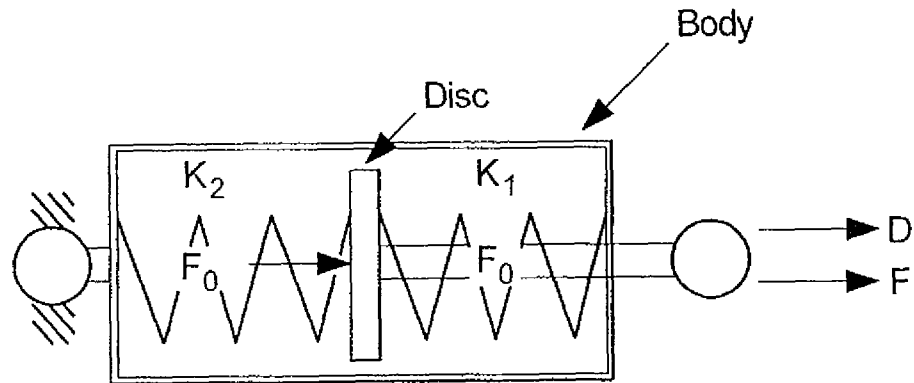
Free-body diagram
