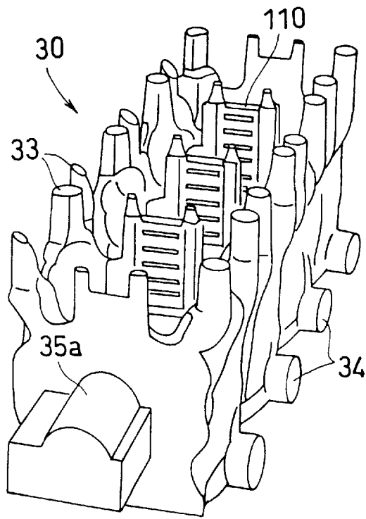
FIG. 8 PRIOR ART
