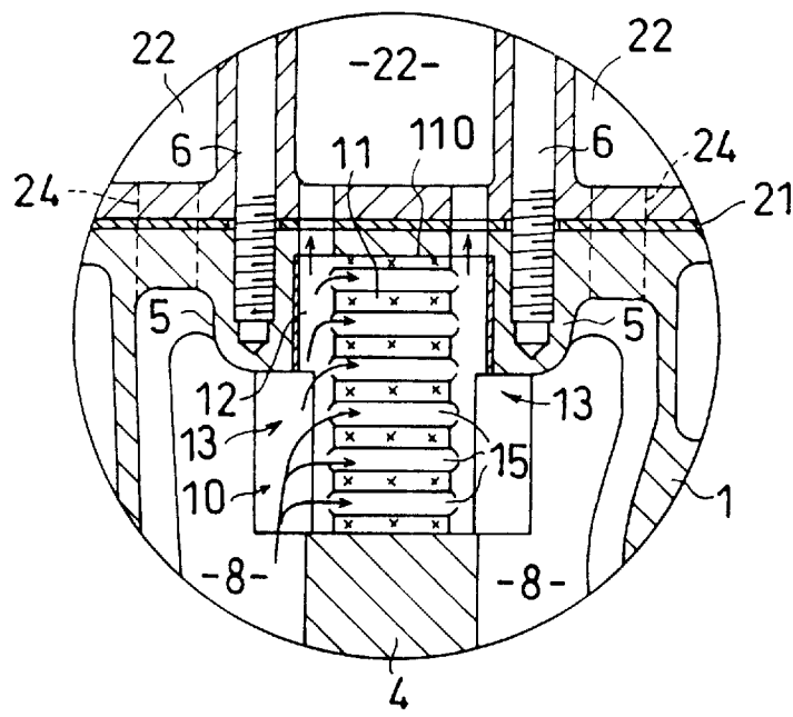
FIG. 7 PRIOR ART
