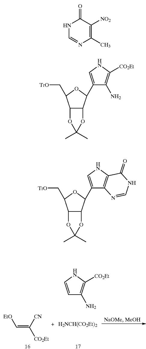
Reaction Scheme 2
