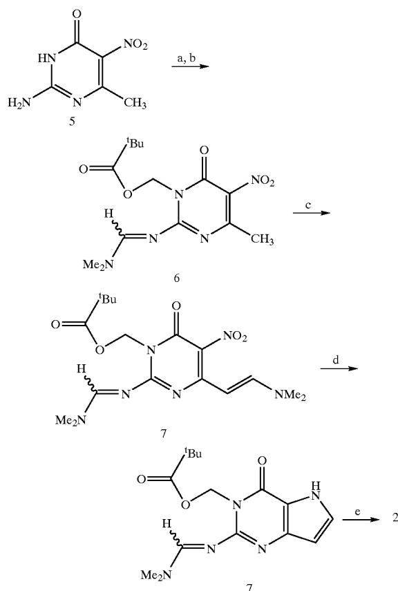
Reaction Scheme 1
