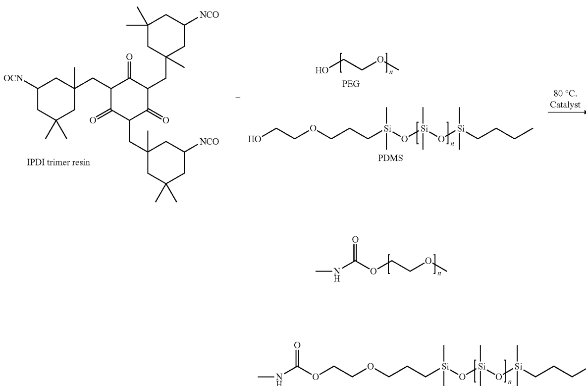
Scheme 1. Synthesis of amphiphilic additive based on IPDI trimer containing PDMS 10,000 \overline{M}_n and PEG 750 \overline{M}_n .
