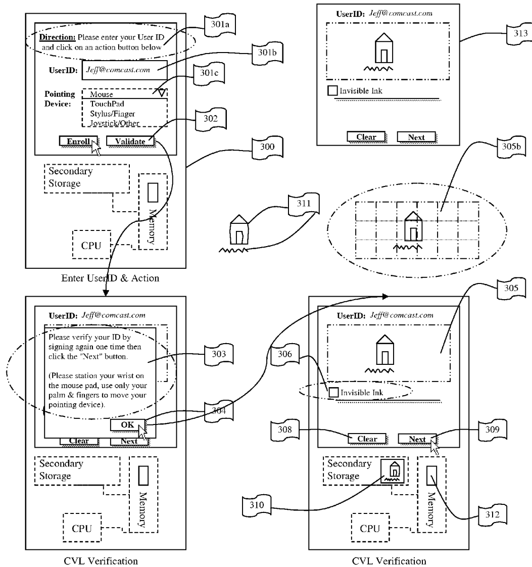
Figure 3: Local Single System CVL Verification.
