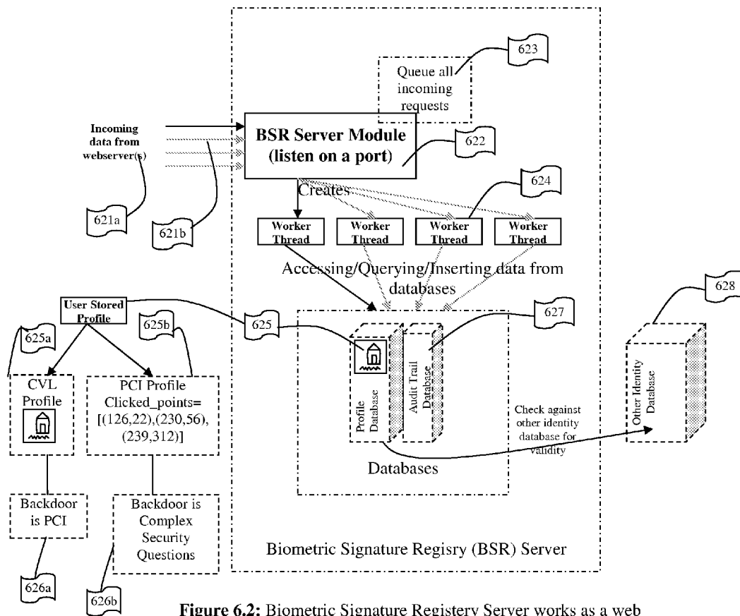
Figure 6.2: Biometric Signature Registry Server works as a web service
