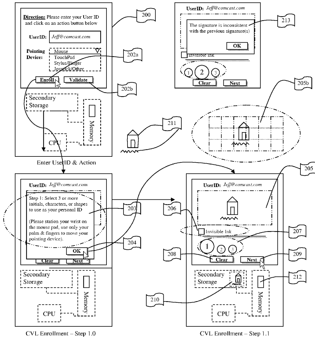
Figure 2: Local Single System CVL Enrollment.
