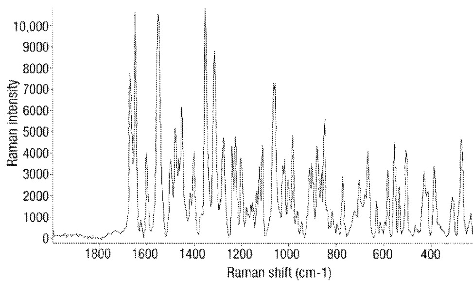
Figure 4: Raman Spectrum of crystal modification A
