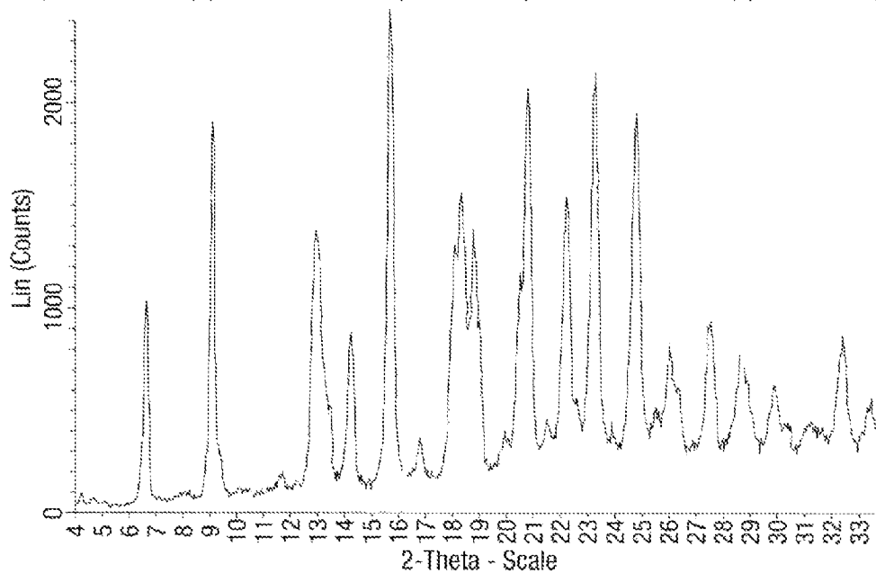
Figure 8: X-ray powder diffraction pattern of crystal modification B (syn/anti: 95:5)
