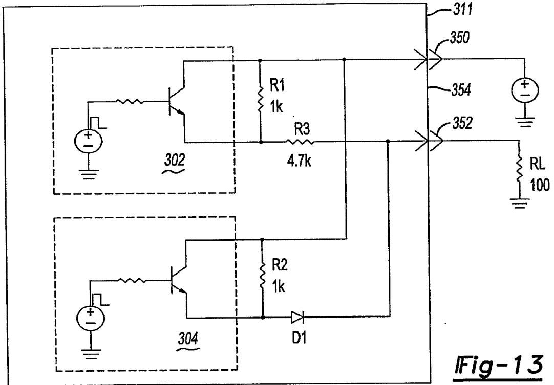
13/29 Sensor Configuration 1
