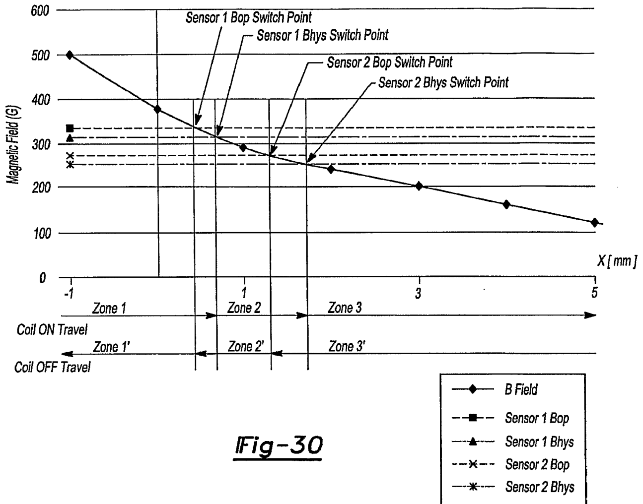
24/29 Sensor Configuration 6 Single Field Operation
