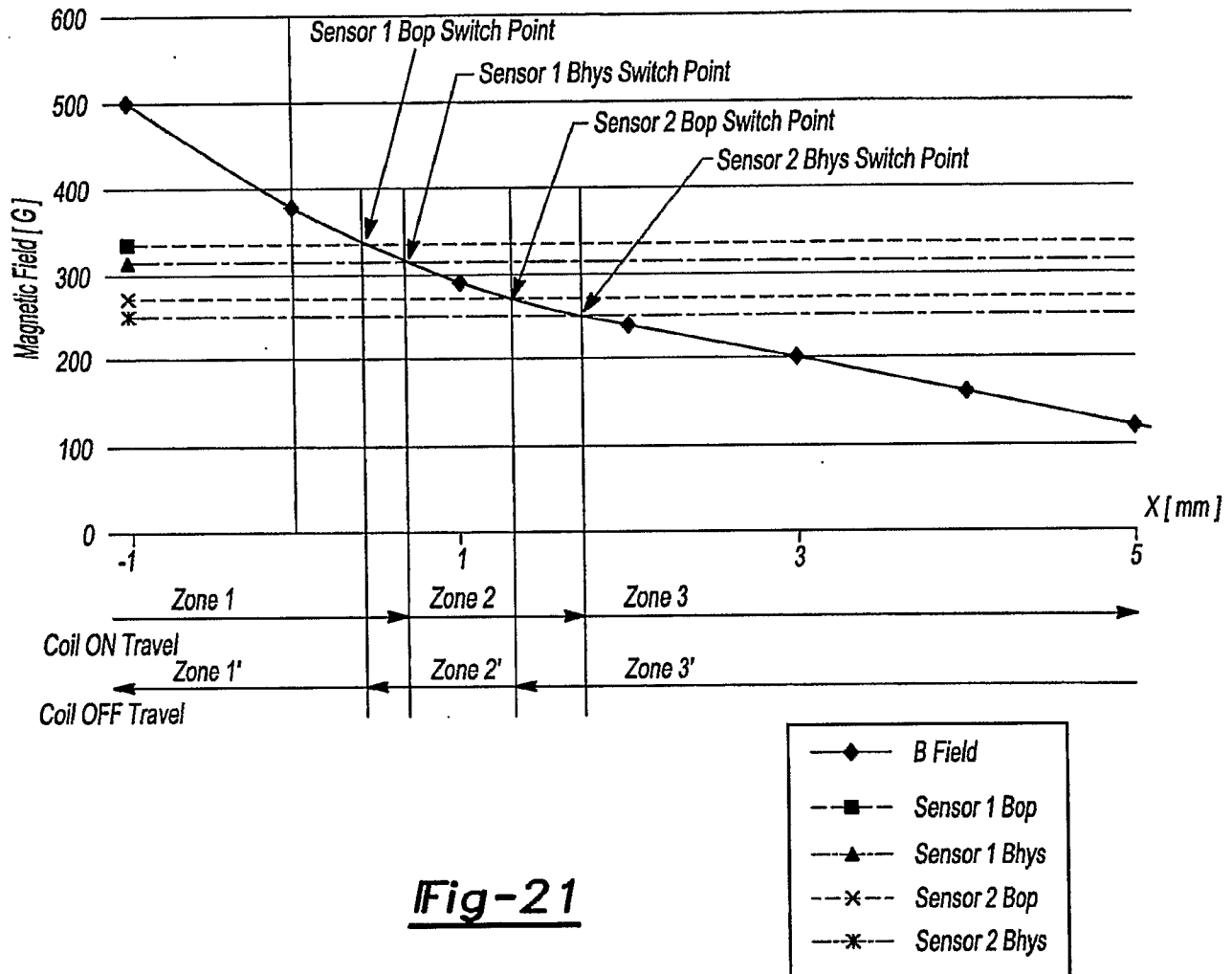
18/29 Sensor Configuration 3 Single Field Operation
