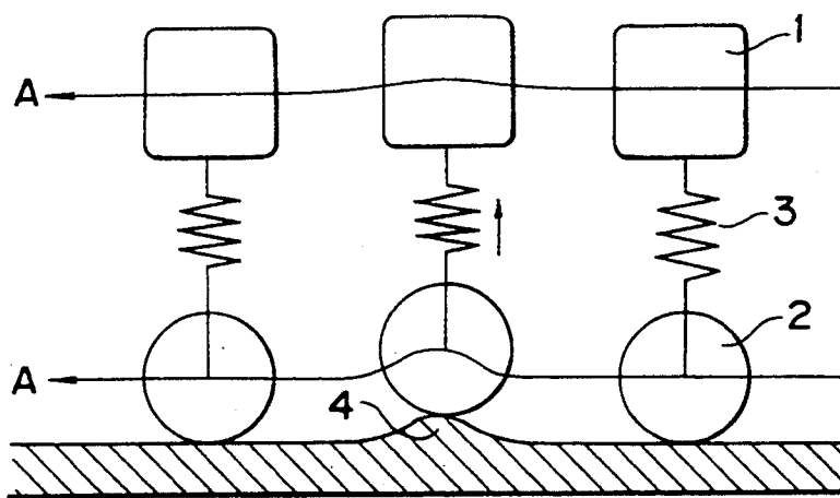
Fig. 22 PRIOR ART
