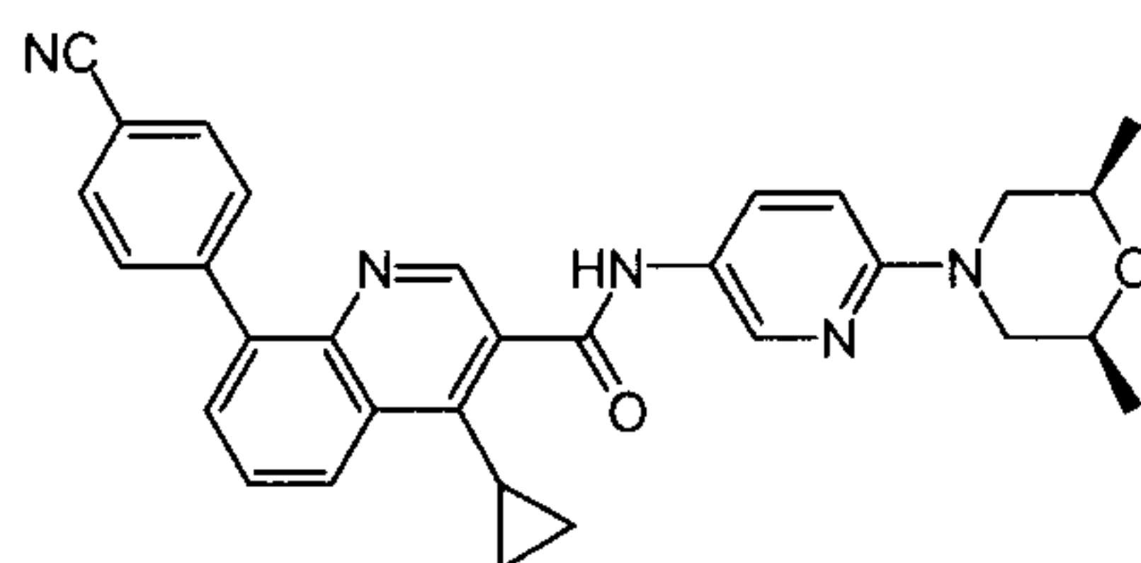
8-(4-cyanophenyl)-4-cyclopropyl-N-(6-((2 S ,6 R )-2,6-dimethylmorpholino)pyridin-3-yl)quinoline-3-carboxamide
