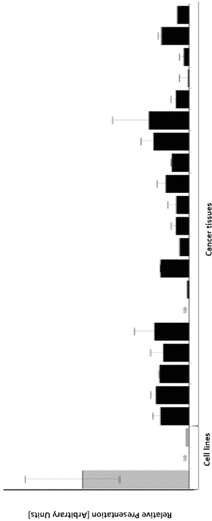
Figure 1S Peptide: ALNPEIVSV (A*02) SEQ ID NO: 148
