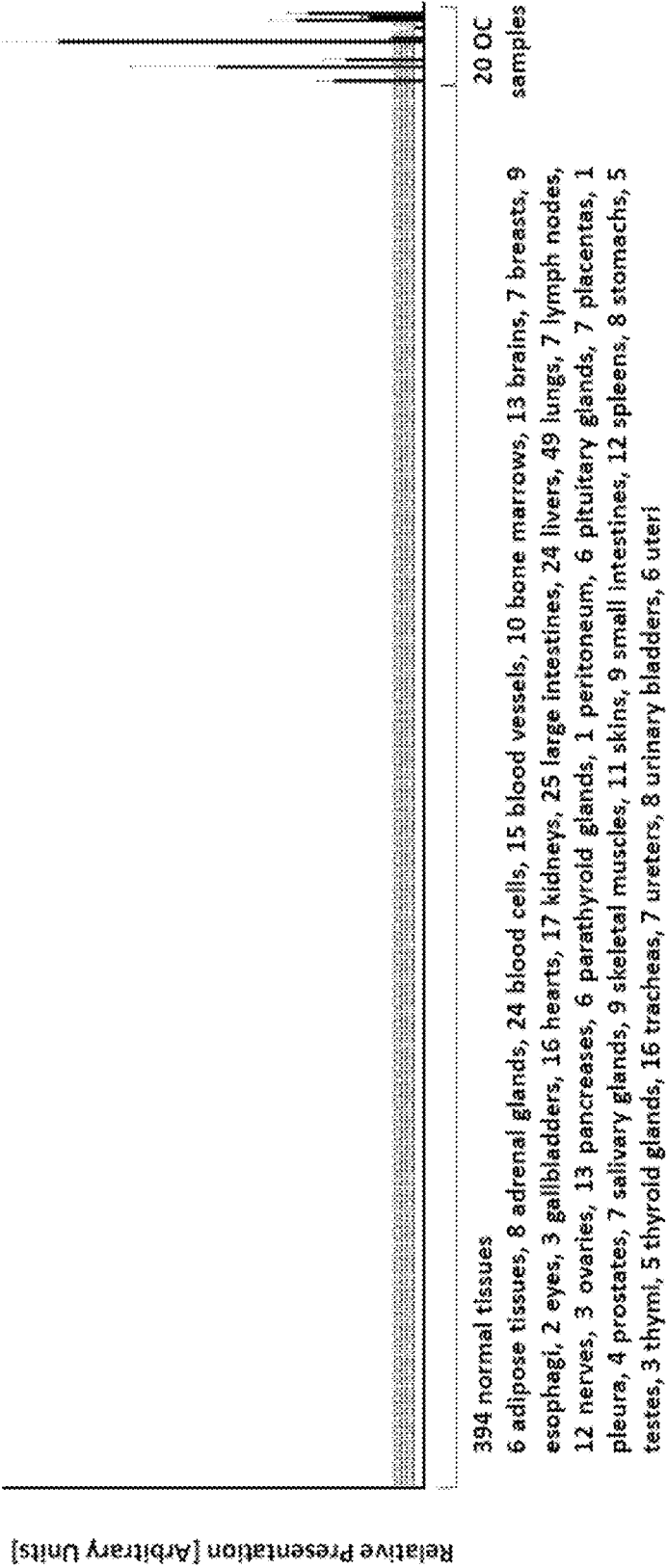
Figure 1H Peptide: SLNDEVPEV (A*02) Seq ID No: 157
