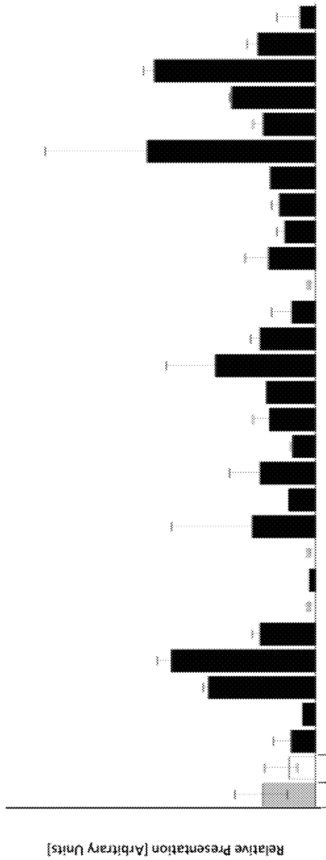
Figure 10 Peptide: FLEDDIHVS (A*02) Seq ID No: 38
