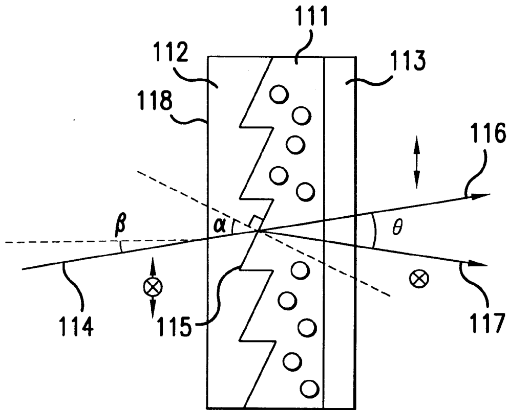
(LIQUID CRYSTAL POLARIZED LIGHT SPLITTING UNIT) 103
