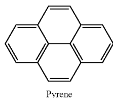
Scheme 2: Structures of tested fluorophores
