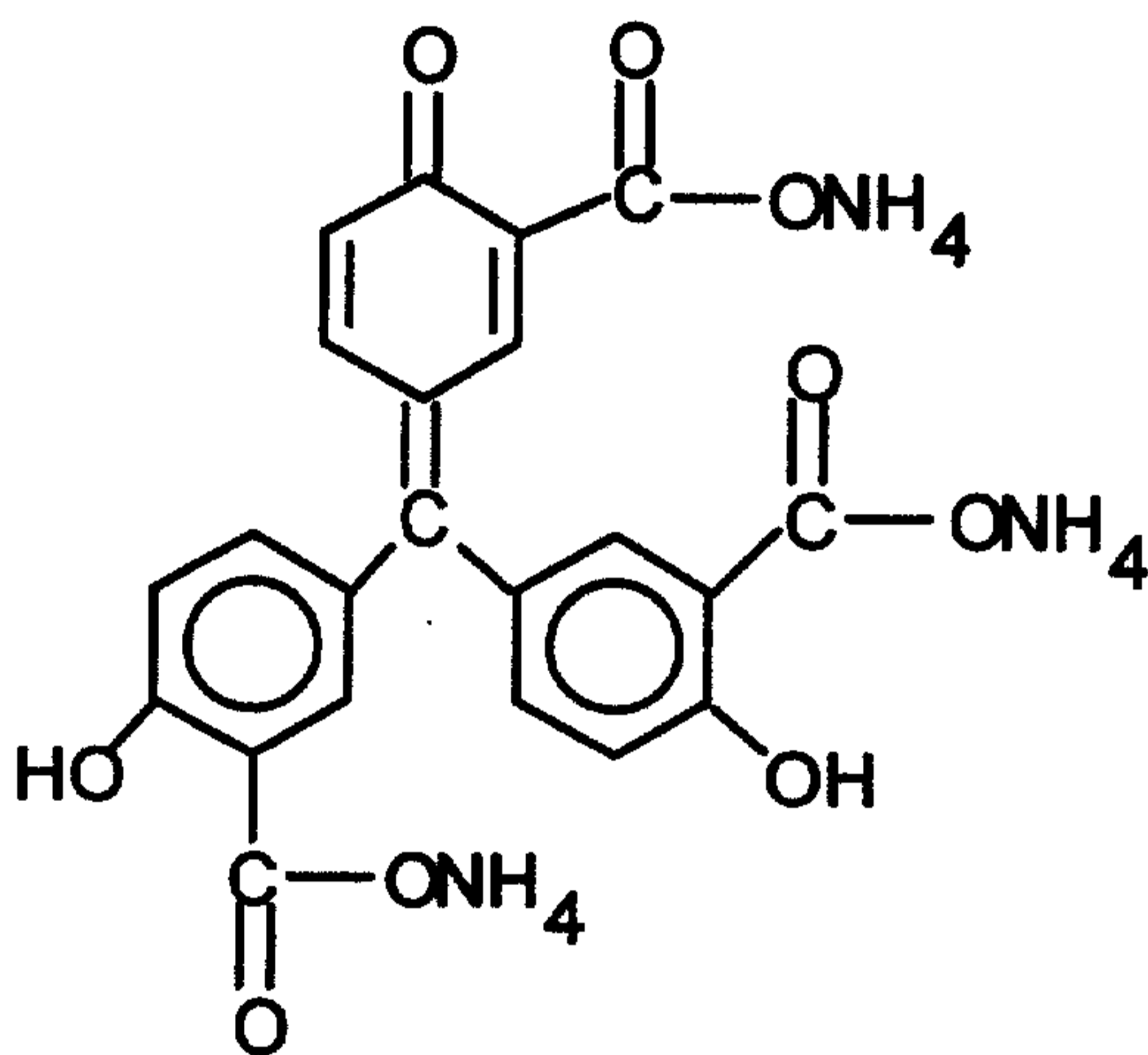
Triammonium Salt
