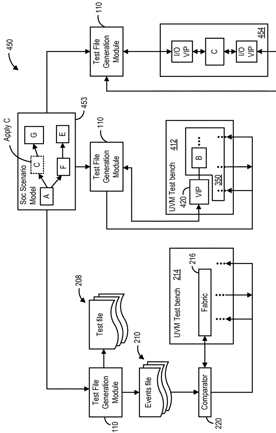
FIG. 4-2 (Multi-level Design Support)
