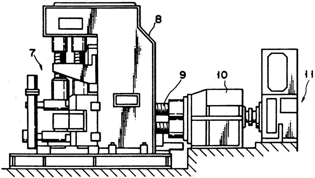
FIG. 10 (PRIOR ART)
