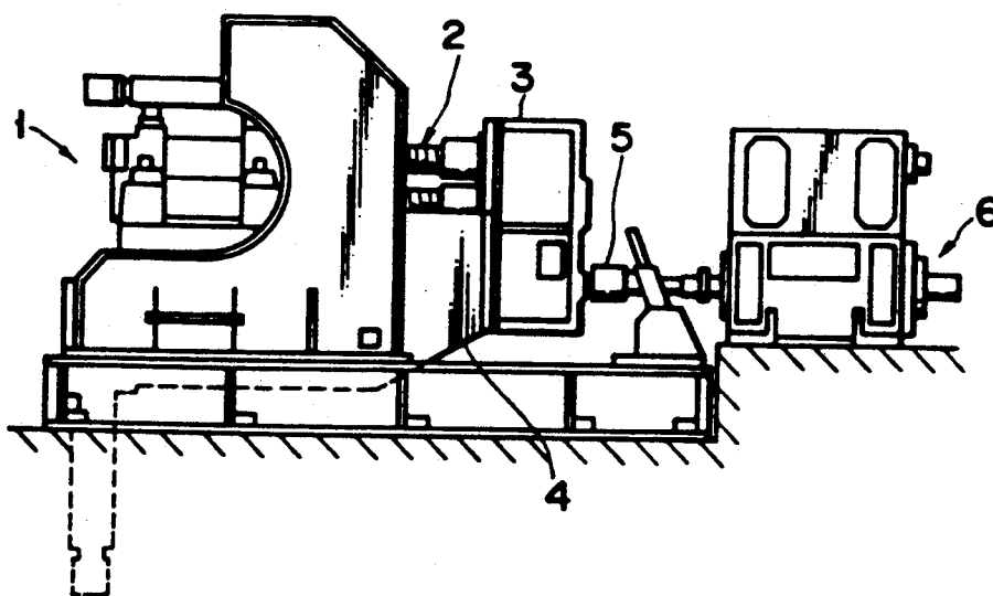
FIG. 9 (PRIOR ART)
