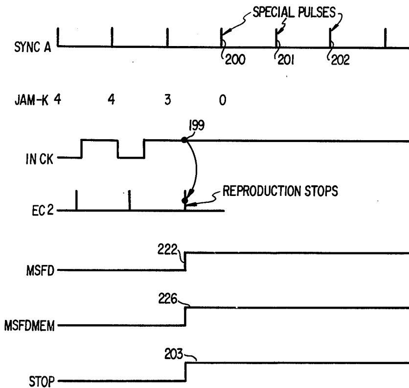
FIG. 7 MISFEED RECOVERY TIMING DIAGRAM
