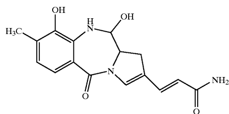
Anthramycin
