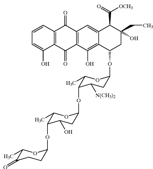
Aclacinomycin A
