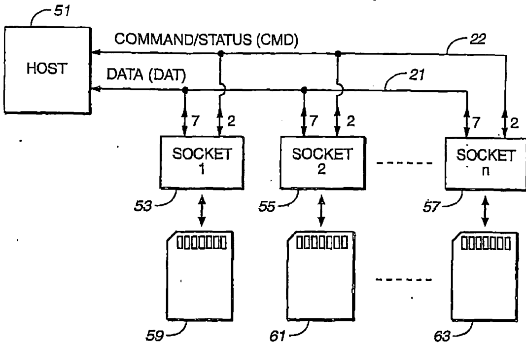
FIG. 3 (PRIOR ART)
