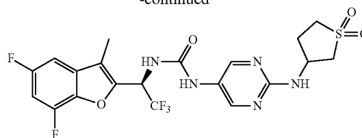
Compound 235
