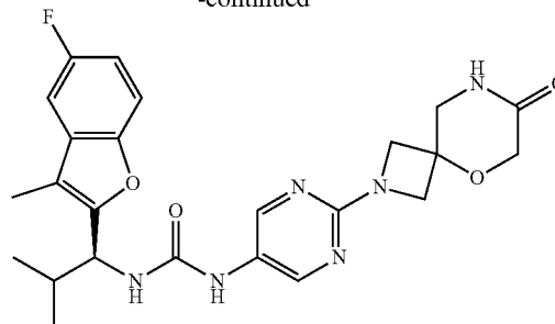
Compound 166
