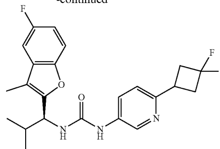
Compound 72
