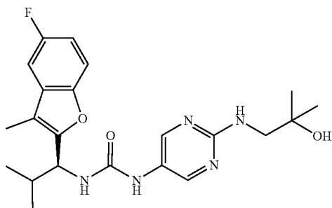
Compound 142
