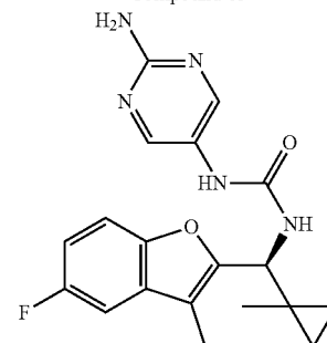
Compound 84
