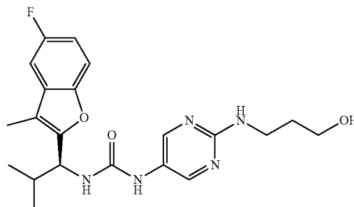
Compound 137
