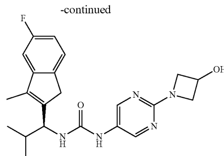
Compound 87
