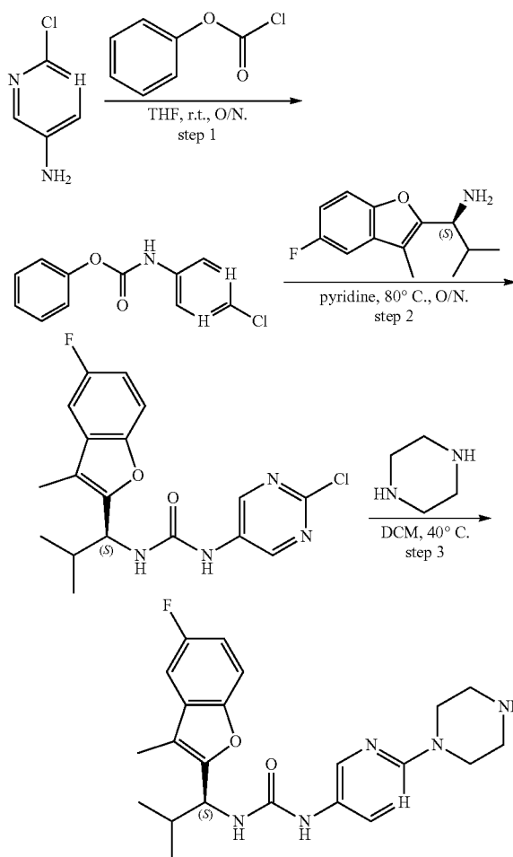
Compound 106
