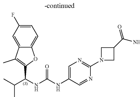
Compound 131
