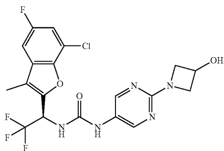
Compound 200
