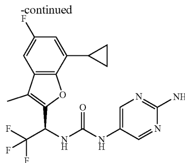
Compound 118
