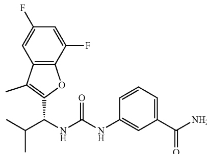
Compound 51
