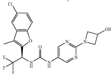
Compound 154
