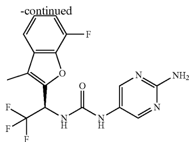
Compound 242
