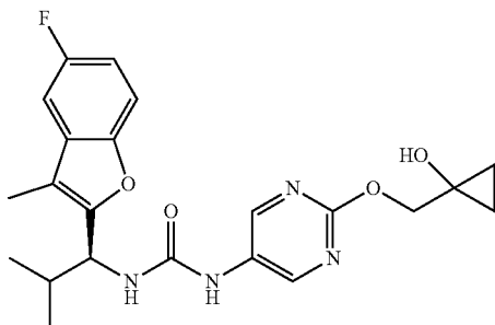
Compound 152
