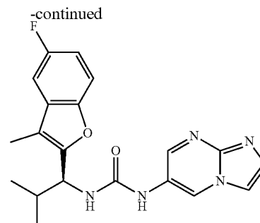
Compound 160
