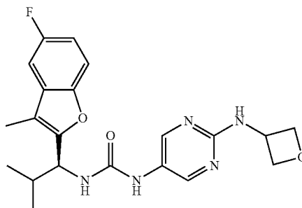
Compound 136
