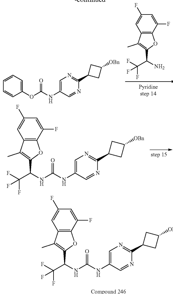
Compound 246
