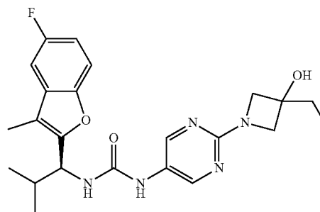
Compound 144
