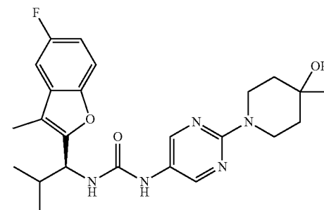
Compound 141
