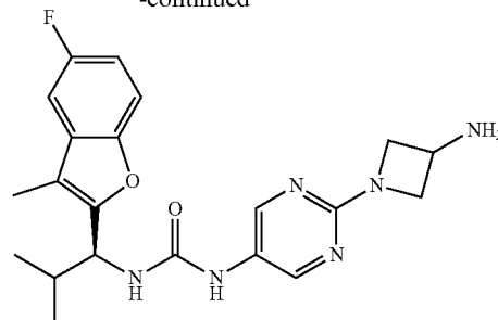
Compound 119
