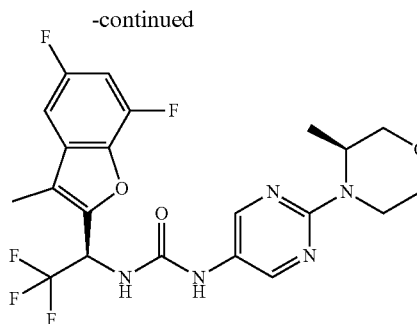
Compound 268
