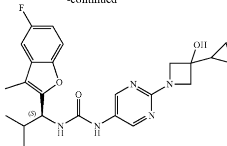
Compound 108
