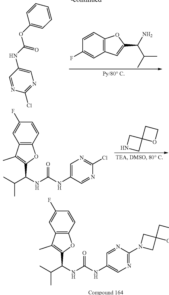
Compound 164
