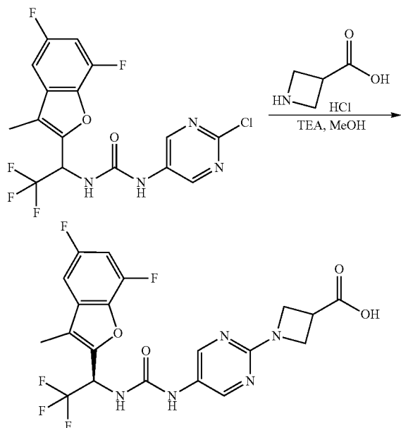
Compound 197
