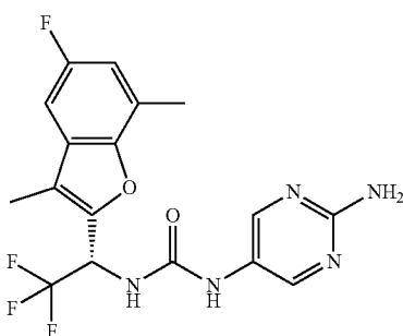
Compound 213
