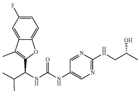
Compound 143
