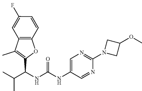
Compound 138
