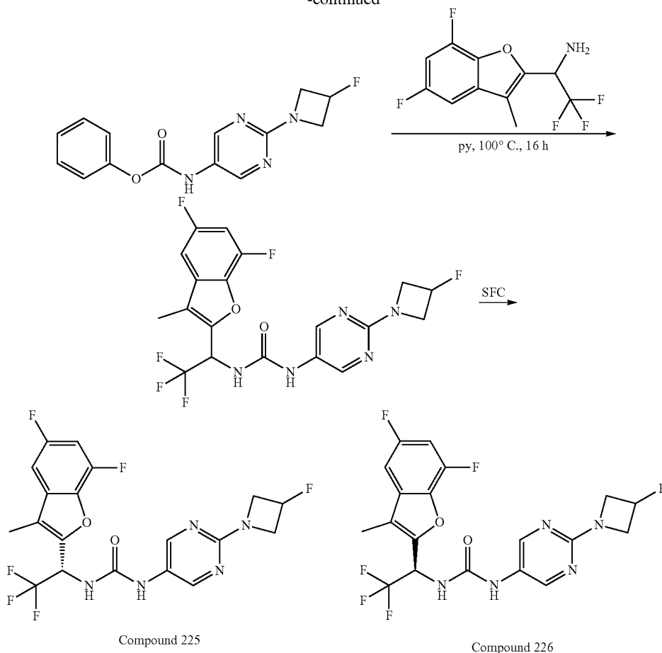
Compound 226
