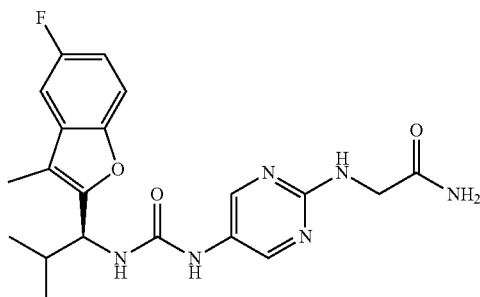
Compound 134
