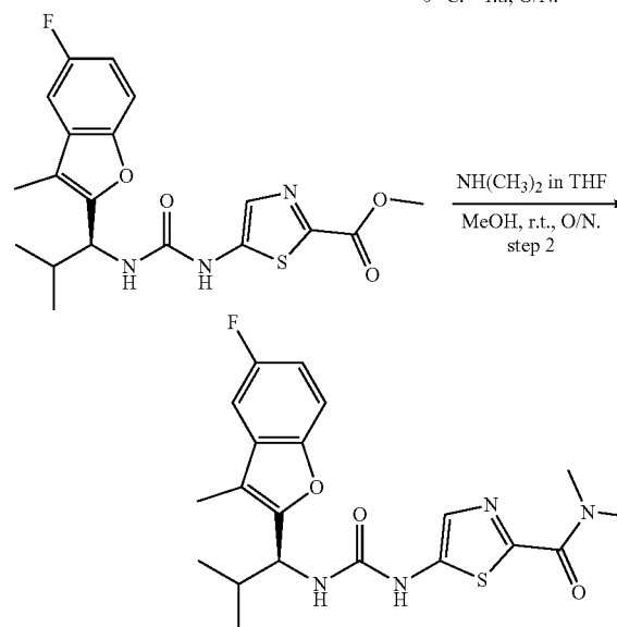
Compound 121
