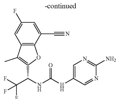
Compound 219
