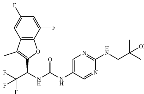
Compound 183
