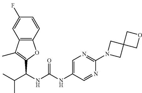
Compound 135
