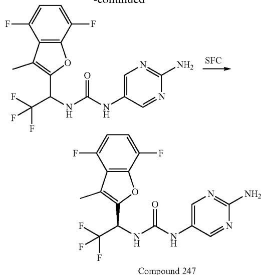
Compound 247
