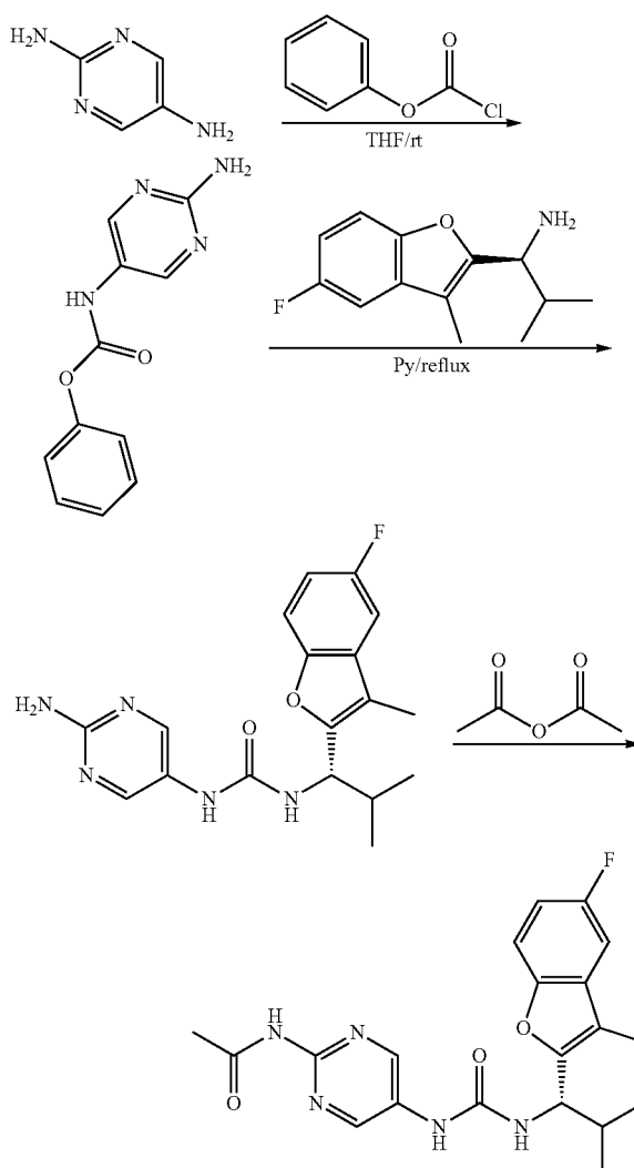
Compound 159
