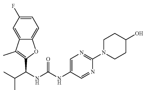
Compound 140
