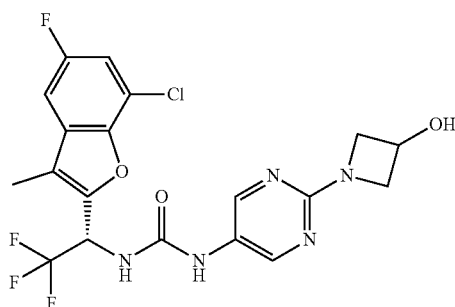
Compound 199
