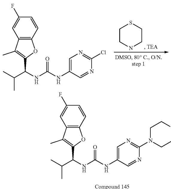
Compound 145
