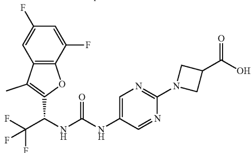
Compound 198
