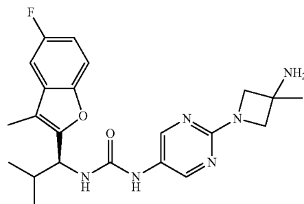
Compound 120
