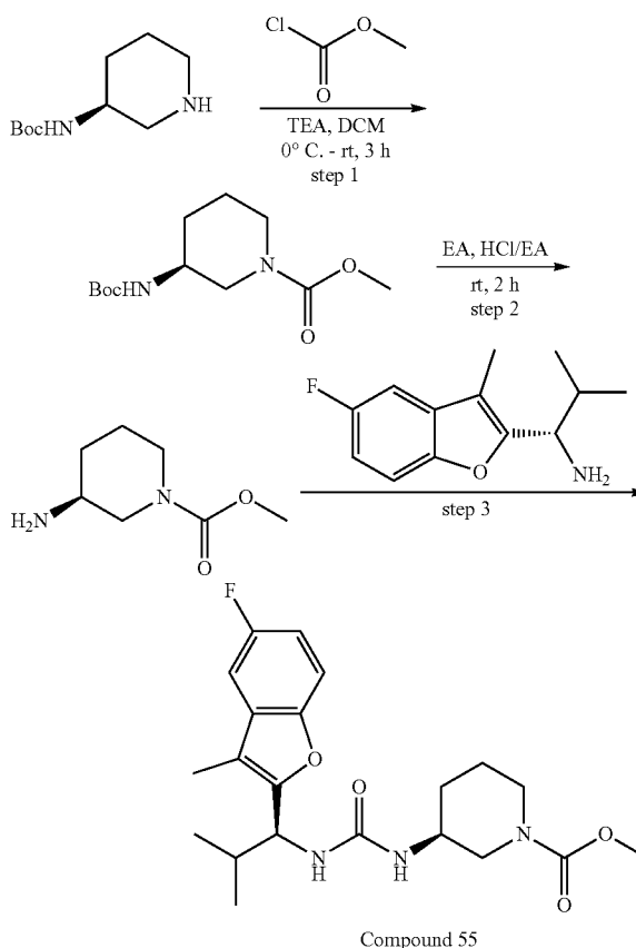
Compound 55
