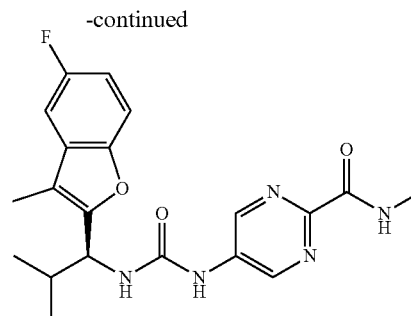
Compound 77
