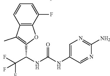
Compound 243
