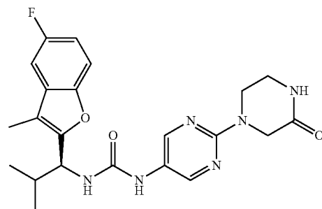
Compound 139
