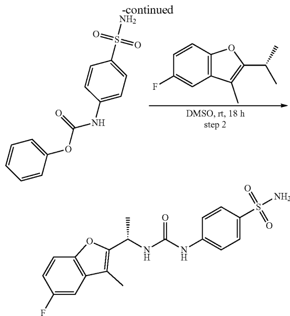
Compound 12
