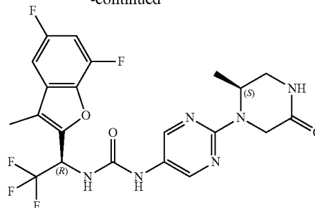
Compound 259
