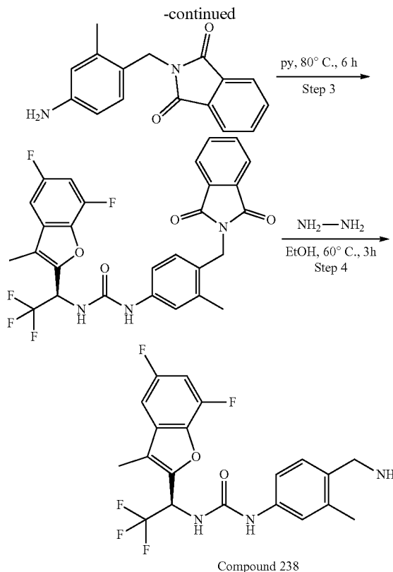
Compound 238
