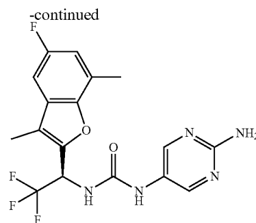
Compound 214
