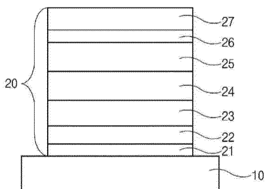
FIG. 1 RELATED ART
