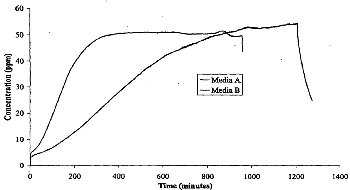
Figure 6 Breakthrough performances of two nanofiber composites
