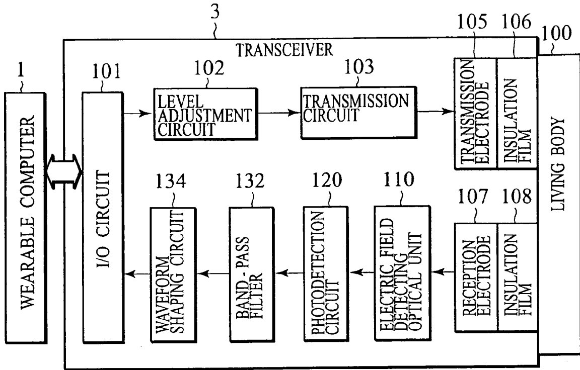
FIG. 4 PRIOR ART
