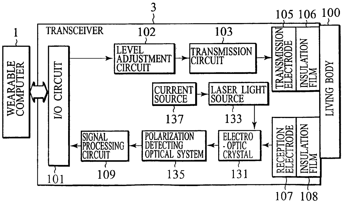
FIG. 3 PRIOR ART
