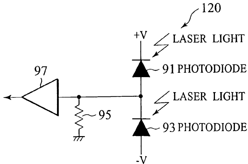
FIG. 5 PRIOR ART
