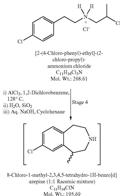
Synthetic Scheme 1.2
