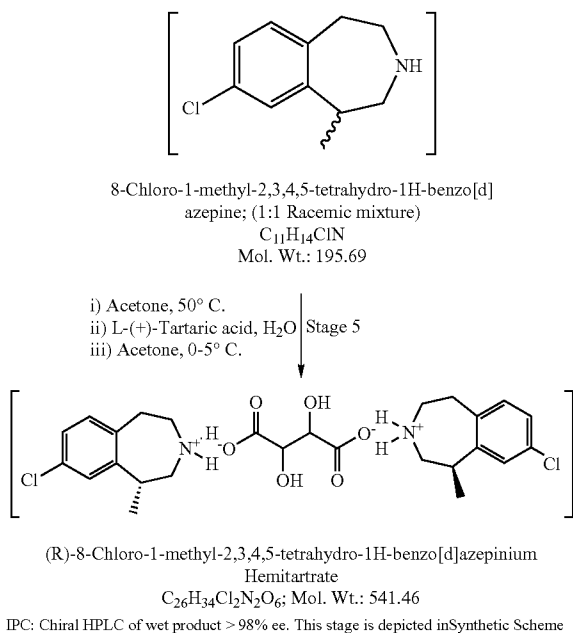
Synthetic Scheme 1.3
