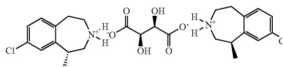
(R)-8-Chloro-1-methyl-2,3,4,5-tetrahydro-1H-benzo[d]azepinium Hemitartrate Final Isolated Intermediate; C 26 H 34 Cl 2 N 2 O 6 Mol. Wt.: 541.46
