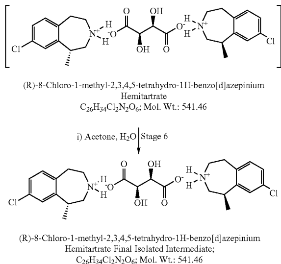
Synthetic Scheme 1.4
