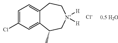
(R)-8-Chloro-1-methyl-2,3,4,5-tetrahydro-1H-benzo[d]azepine Hemihydrate C 11 H 15 Cl 2 N. 0.5 H 2 O Mol. Wt.: 241.16
