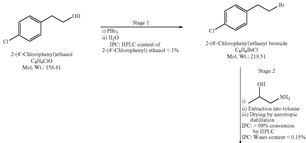
Synthetic Scheme 1.1
