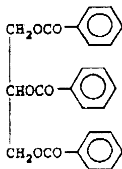
Compound 12
