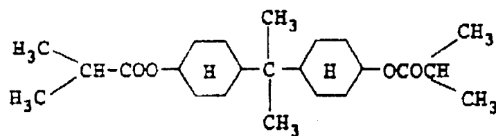
Compound 29
