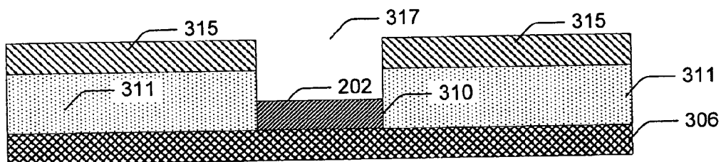
Etch Passivation Insulator Layer in Tunnel Junction Regions
