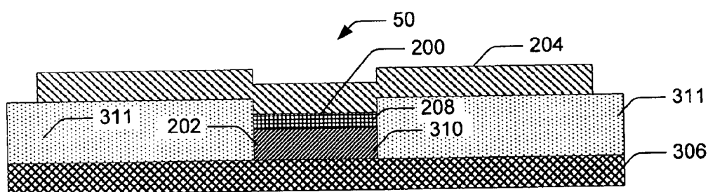
Following Imprint Process, Pattern and Form Second Superconductor Electrodes
