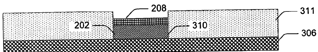
Oxidize Exposed Superconductor Metal to Form Tunnel Barrier
