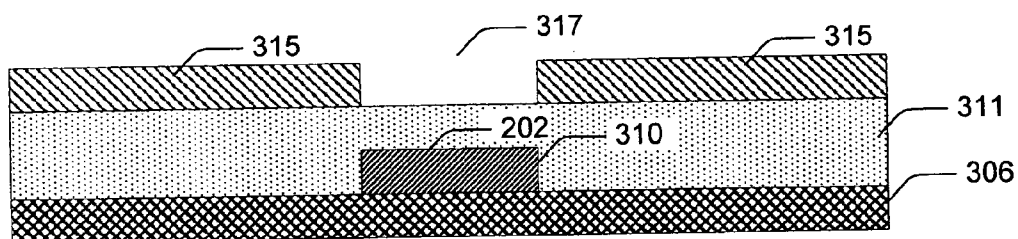
Lift - Off Hard Mask Imprint Layer Leaving Hard Mask Metal Behind
