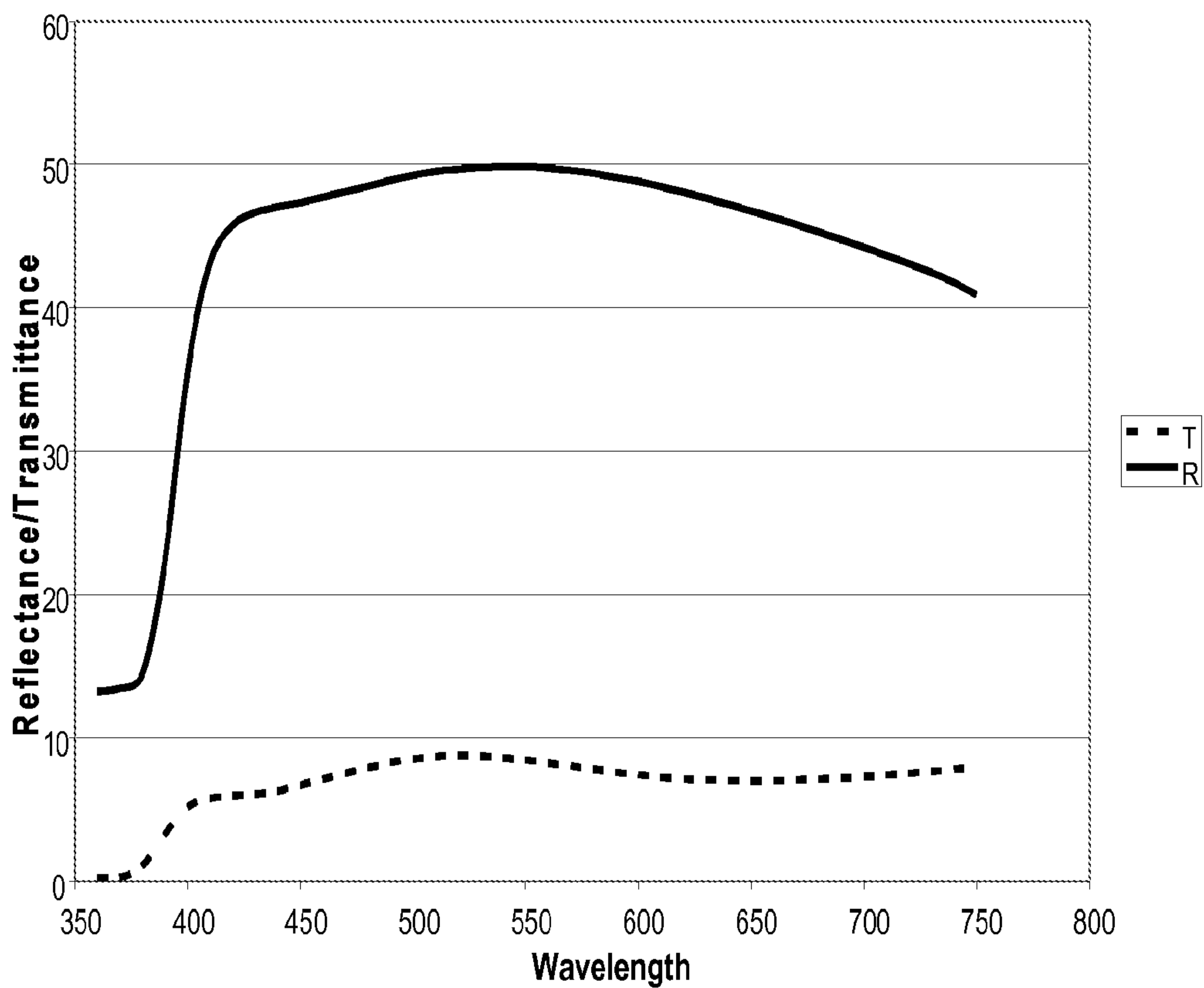
Option 5: Glass/ 3/4 wave ITO/Cr/Ru
