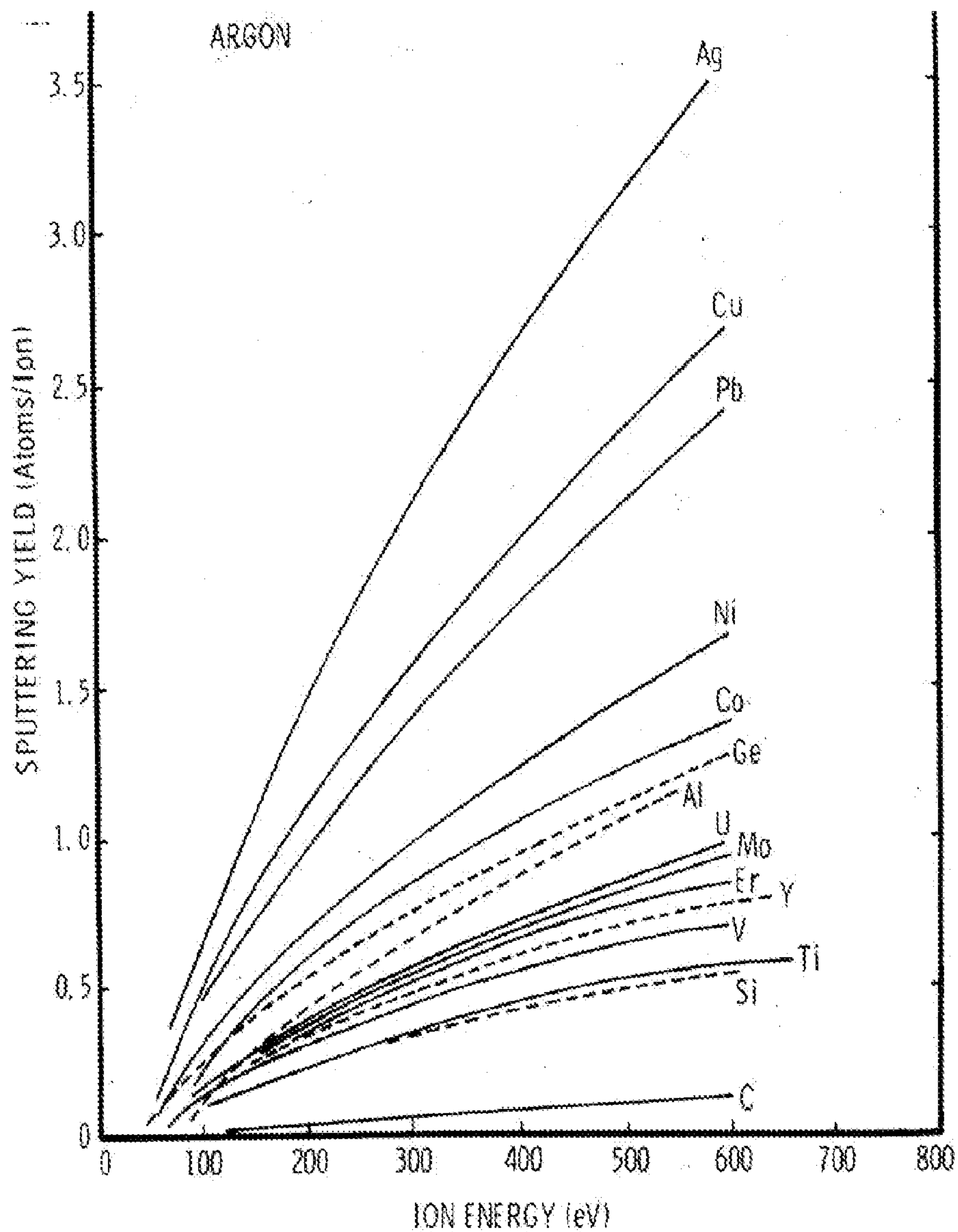
Figure 5.5: Variation of sputtering yield with ion energy at normal angle of incidence. Data from R.V. Stuart and G.K. Wehner, J. Appl. Phys. 33, 2351 (1962); D. Rosenberg and G.K. Wehner, J. Appl. Phys. 33, 1842 (1962); R. Behrisch, Ergeb. Exakt. Naturw. 35, 295 (1964).
