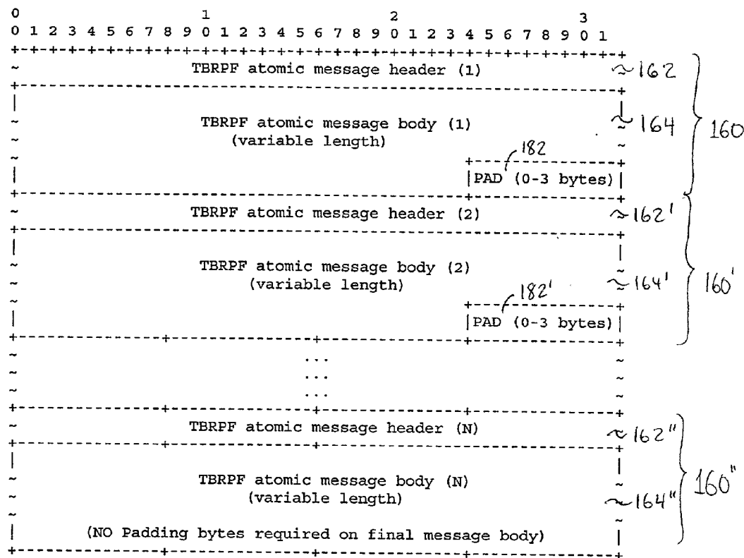
FIG. 7 (A COMPOUND TBRPF MESSAGE)
