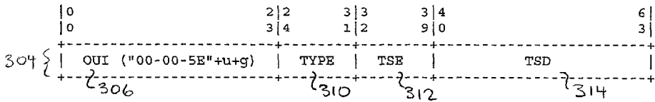
FIG. 15C Interface Identifier format for IANA
