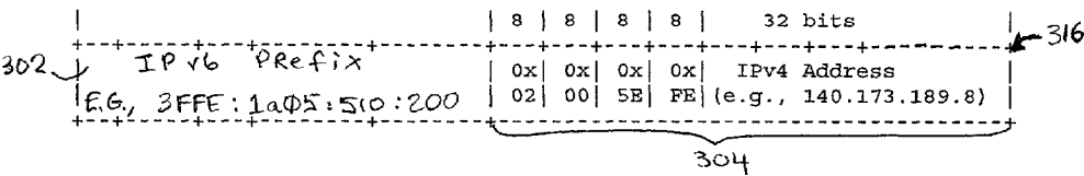
FIG. 15D IPv6-IPv4 Compatibility Address
