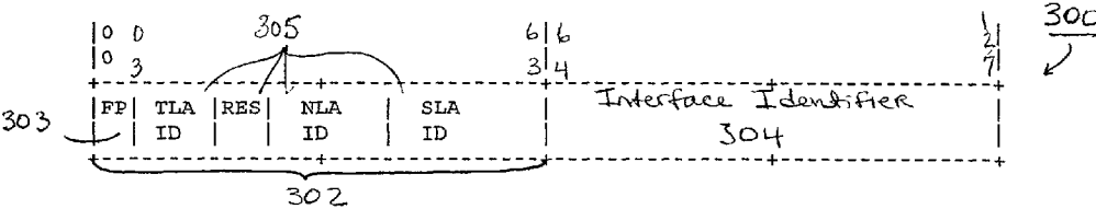
FIG. 15A IPv6-IPv4 Compatibility Address Format
