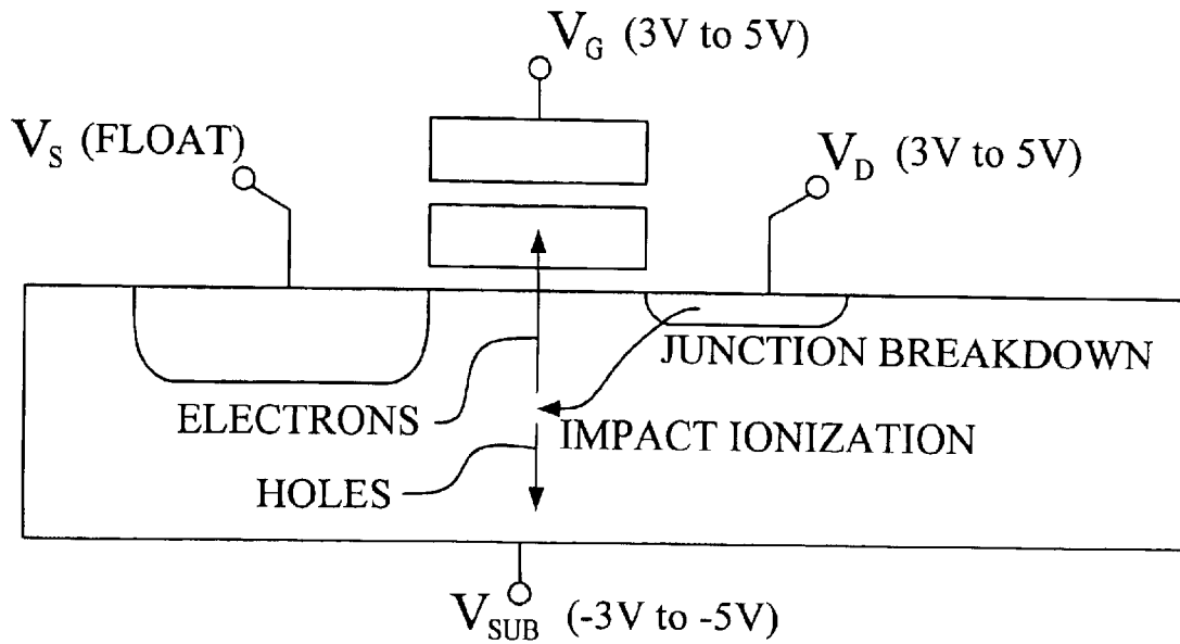
FIG. 9 BACK BIAS HOT ELECTRON INJECTION PROGRAMMING MECHANISM
