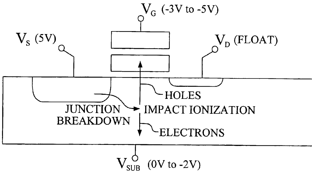
FIG. 10 BACK BIAS HOT HOLE INJECTION ERASE MECHANISM
