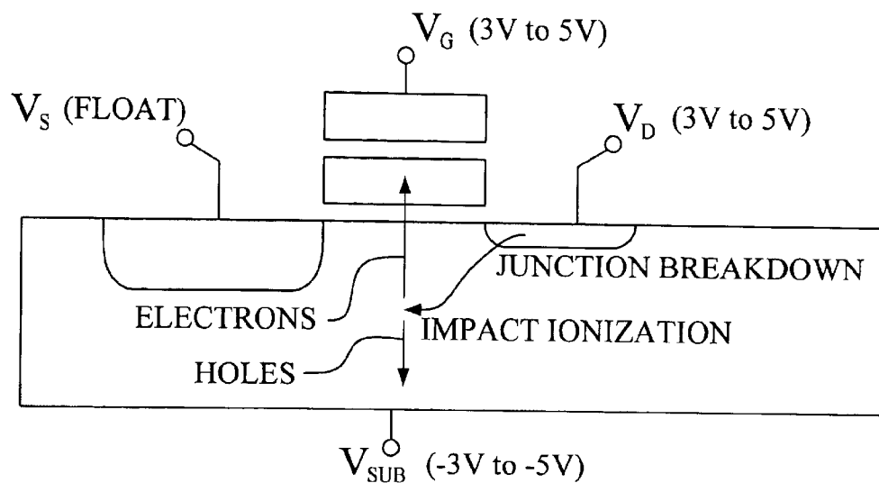
BACK BIAS HOT ELECTRON INJECTION PROGRAMMING MECHANISM
